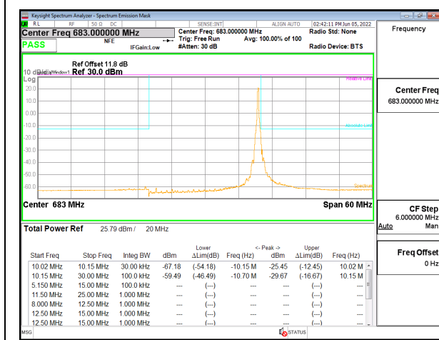
5G NR n71 20MHz BPSK Middle Channel RB1-105
