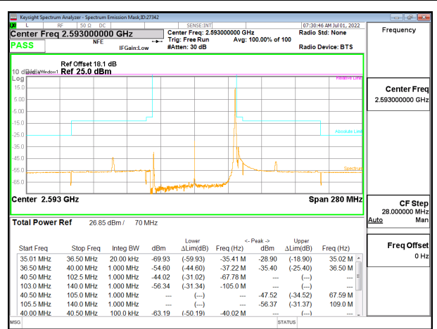
5G NR n41 70MHz BPSK Middle Channel RB1-188
