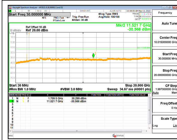
5G NR n70 5MHz BPSK High Channel RB1-24
