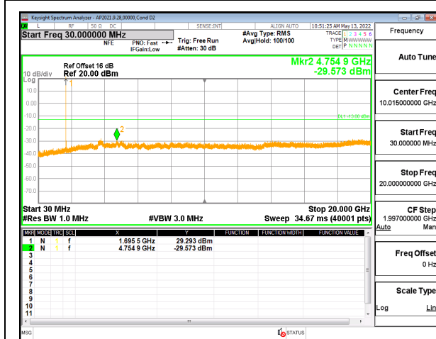
5G NR n70 15MHz BPSK Middle Channel RB1-1
