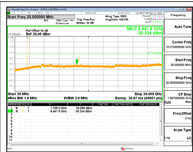
5G NR n70 10MHz BPSK High Channel RB1-1
