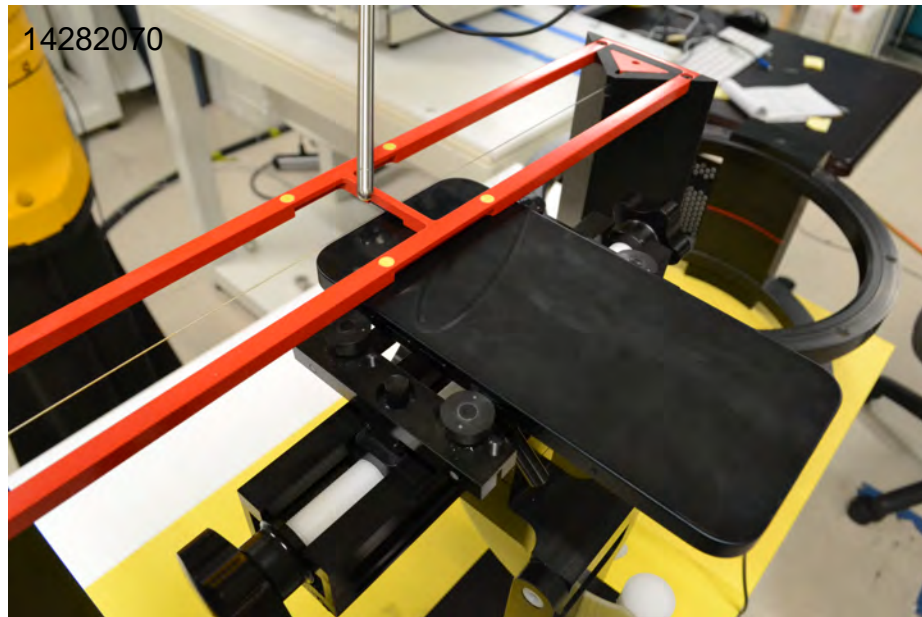
Photograph 2: Front View of the DUT SAR 9
