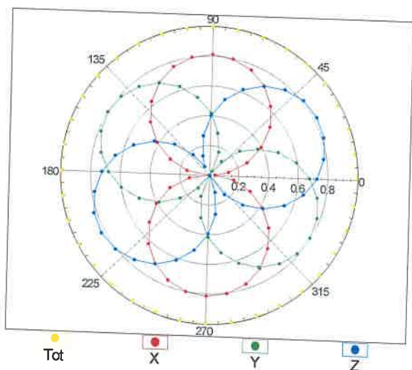
f=600 MHz,TEM
