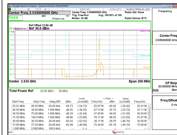
5G NR n7 50MHz BPSK Middle Channel RB1-215
