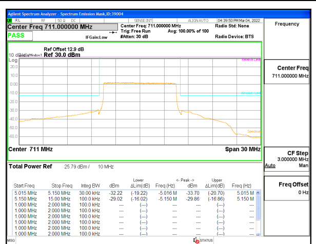
LTE B12 10MHz QPSK High Channel RB50-0
