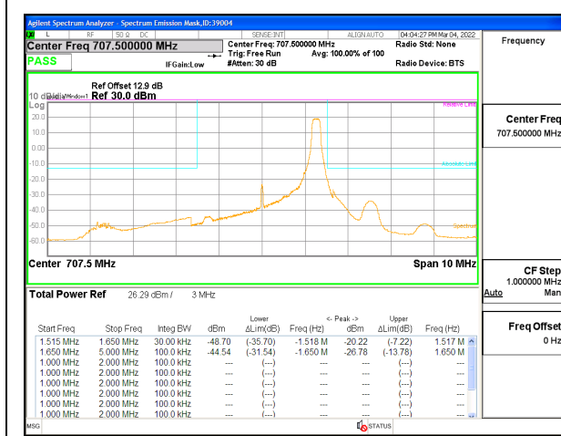
LTE B12 3MHz QPSK Middle Channel RB1-14
