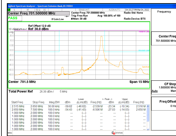
LTE B12 5MHz QPSK Low Channel RB1-24
