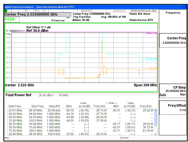
5G NR n7 50MHz BPSK Low Channel RB1-269
