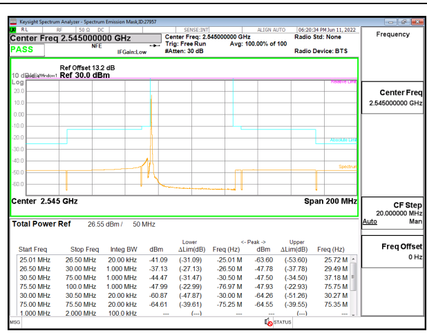
5G NR n7 50MHz BPSK High Channel RB1-0
