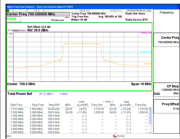
LTE B12 3MHz QPSK Low Channel RB15-0
