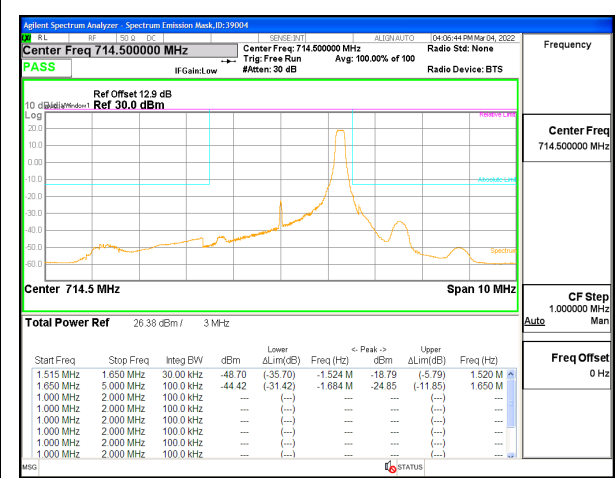
LTE B12 3MHz QPSK High Channel RB1-14
