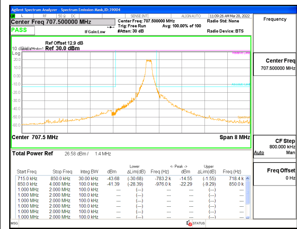
LTE B12 1.4MHz QPSK Middle Channel RB1-5
