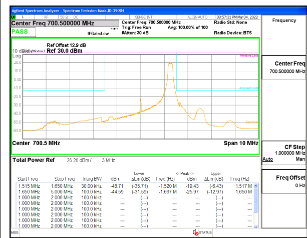
LTE B12 3MHz QPSK Low Channel RB1-14
