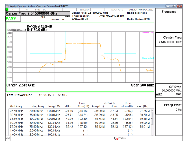
5G NR n7 50MHz BPSK High Channel RB270-0
