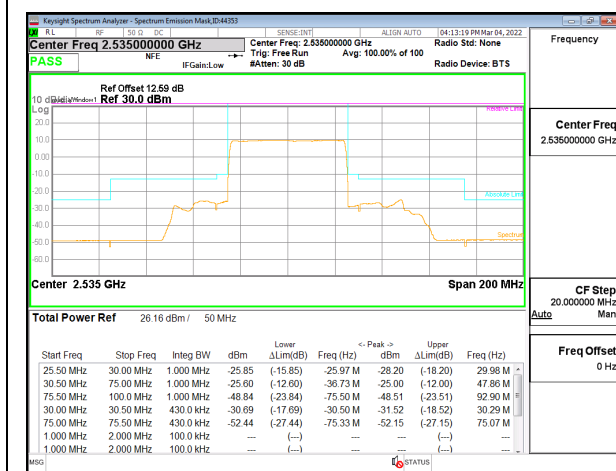
5G NR n7 50MHz BPSK Middle Channel RB216-0
