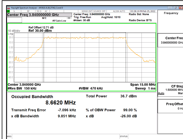
5G NR n77 10MHz BPSK Middle Channel RB14-0
