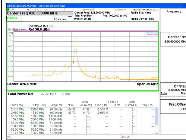
LTE B5 5MHz QPSK Low Channel RB1-0: ID 52275
