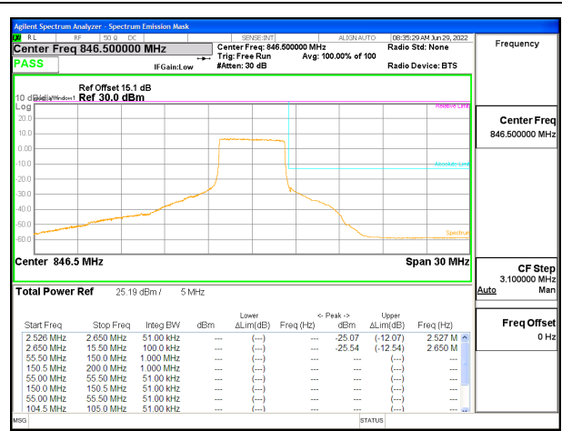
LTE B5 5MHz QPSK High Channel RB25-0: ID 52275
