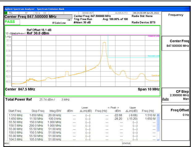
LTE B5 3MHz QPSK High Channel RB1-14: ID 52275
