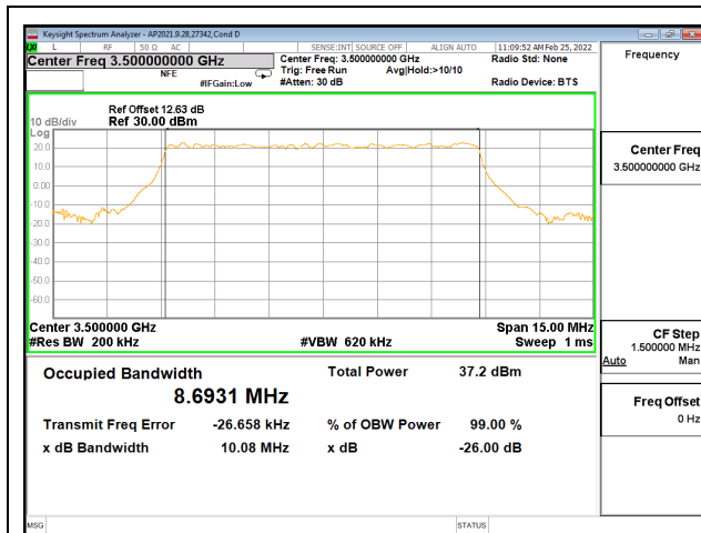
5G NR n77 10MHz BPSK Middle Channel RB14-0
