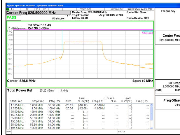
LTE B26 3MHz QPSK Low Channel RB15-0: ID 52275
