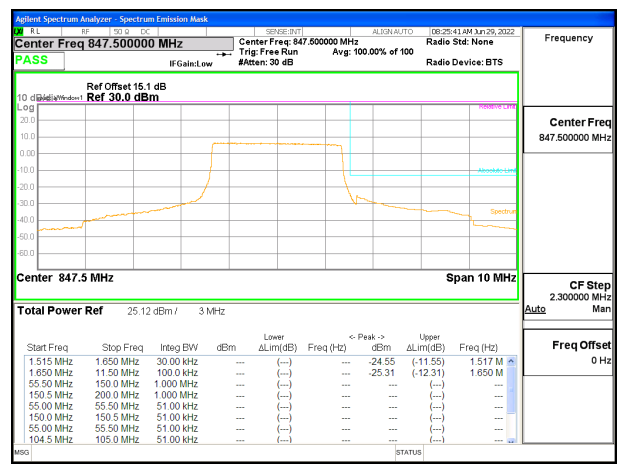
LTE B5 3MHz QPSK High Channel RB15-0: ID 52275
