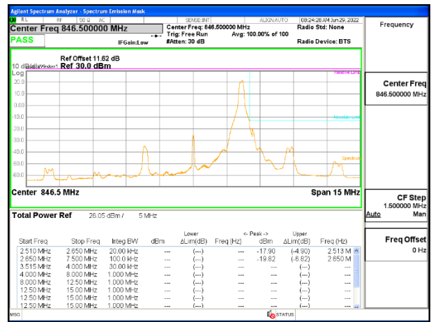
5G NR n5 5MHz BPSK High Channel RB1-24: ID 52275
