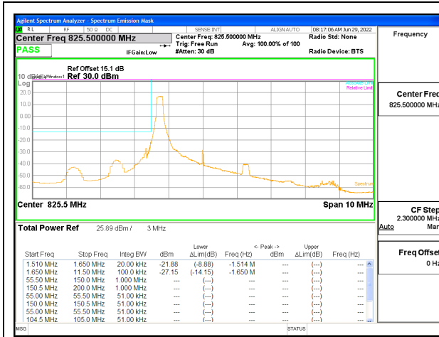
LTE B5 3MHz QPSK Low Channel RB1-0: ID 52275
