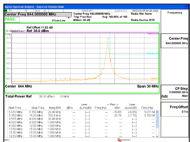
5G NR n5 10MHz BPSK High Channel RB1-51: ID 52275
