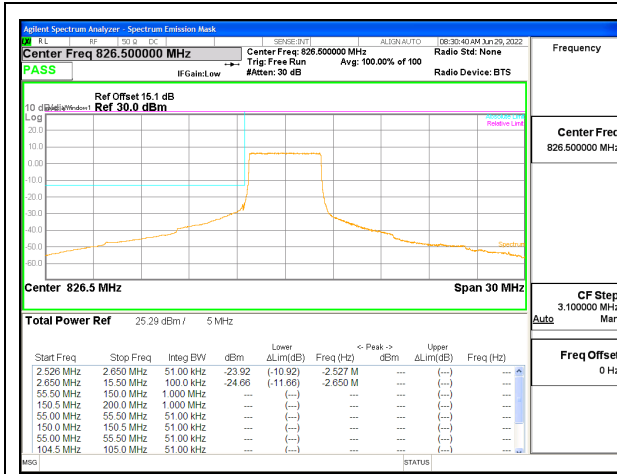
LTE B5 5MHz QPSK Low Channel RB25-0: ID 52275
