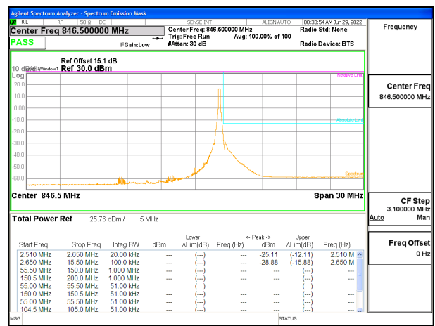
LTE B5 5MHz QPSK High Channel RB1-24: ID 52275
