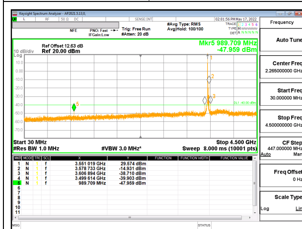
5G NR n48 30MHz BPSK Low Channel RB1-0 (30MHz to 4.5GHz) , ID:52275
