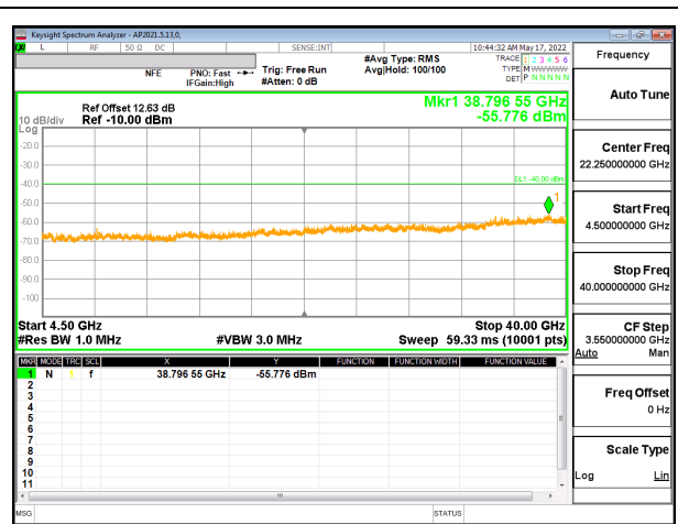
5G NR n48 20MHz BPSK High Channel RB1-50 (4.5G to 40G) , ID:52275
