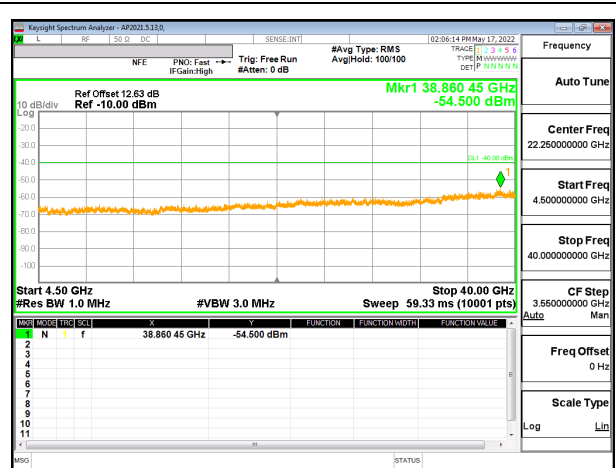
5G NR n48 30MHz BPSK Low Channel RB1-0 (4.5G to 40G) , ID:52275
