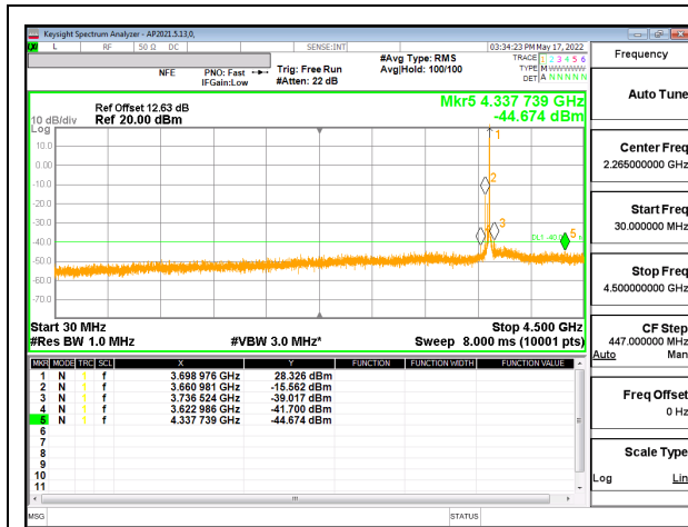
5G NR n48 40MHz BPSK High Channel RB1-105 (30MHz to 4.5GHz) , ID:52275
