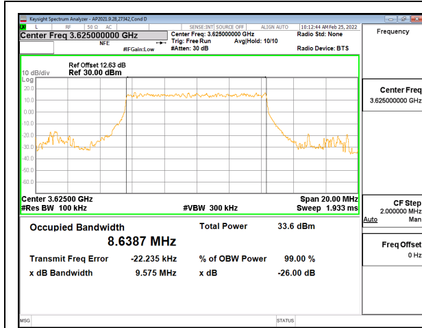
5G NR n48 10MHz BPSK Middle Channel RB25-0
