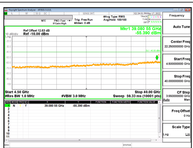
5G NR n48 30MHz BPSK High Channel RB1-1 (4.5G to 40G) , ID:52275
