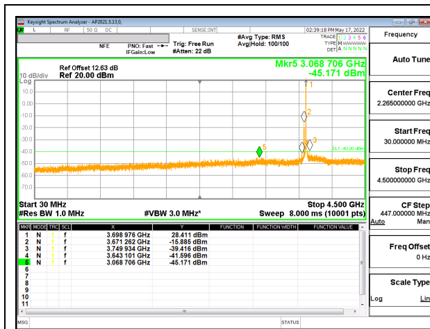
5G NR n48 30MHz BPSK High Channel RB1-1 (30MHz to 4.5GHz) , ID:52275
