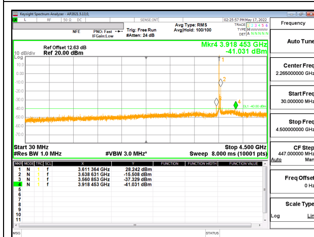
5G NR n48 30MHz BPSK High Channel RB1-1 (30MHz to 4.5GHz) , ID:52275
