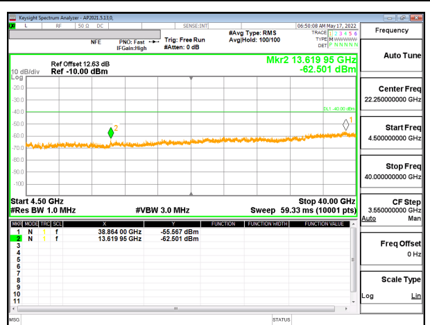
5G NR n48 10MHz BPSK Mid Channel RB1-1 (4.5G to 40G), ID:52275
