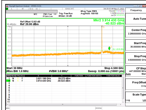
5G NR n48 10MHz BPSK Mid Channel RB1-1 (30MHz to 4.5GHz), ID:52275
