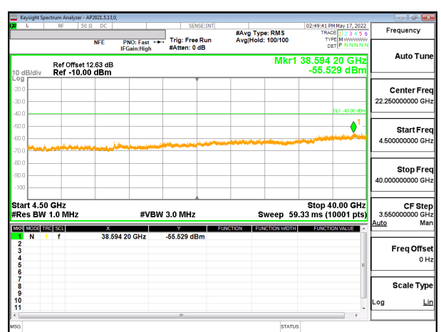
5G NR n48 40MHz BPSK Low Channel RB1-0 (4.5G to 40G) , ID:52275
