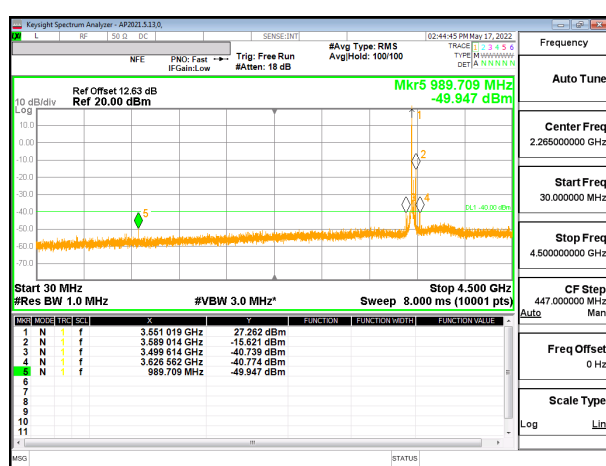
5G NR n48 40MHz BPSK Low Channel RB1-0 (30MHz to 4.5GHz) , ID:52275
