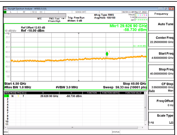
5G NR n48 10MHz BPSK Low Channel RB1-0 (4.5G to 40G), ID:52275
