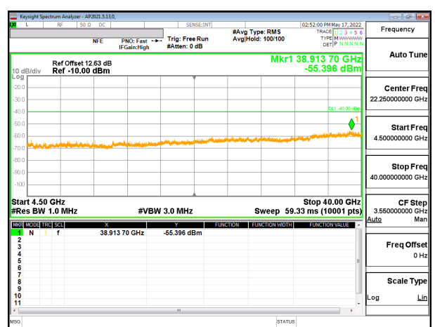
5G NR n48 40MHz BPSK Middle Channel RB1-1 (4.5G to 40G) , ID:52275
