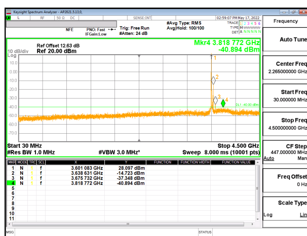
5G NR n48 40MHz BPSK Mid Channel RB1-1 (30MHz to 4.5GHz) , ID:52275
