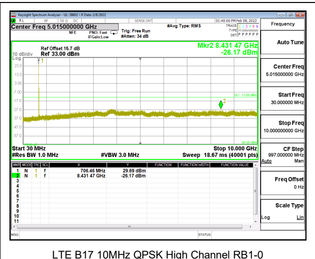
LTE B17 10MHz QPSK High Channel RB1-0
