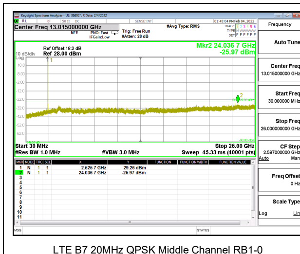
LTE B7 20MHz QPSK Middle Channel RB1-0
