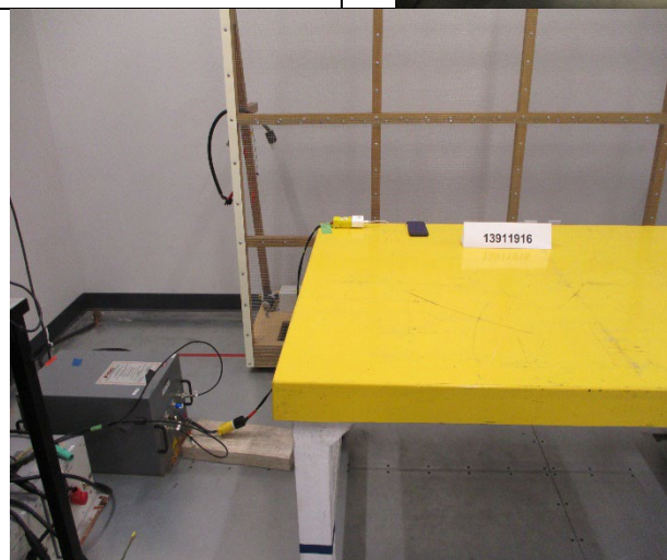
AC LINE CONDUCTED (FRONT)
