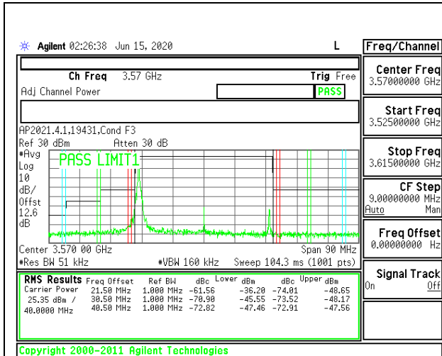
5G NR n48 40MHz BPSK Low Channel RB1-0
