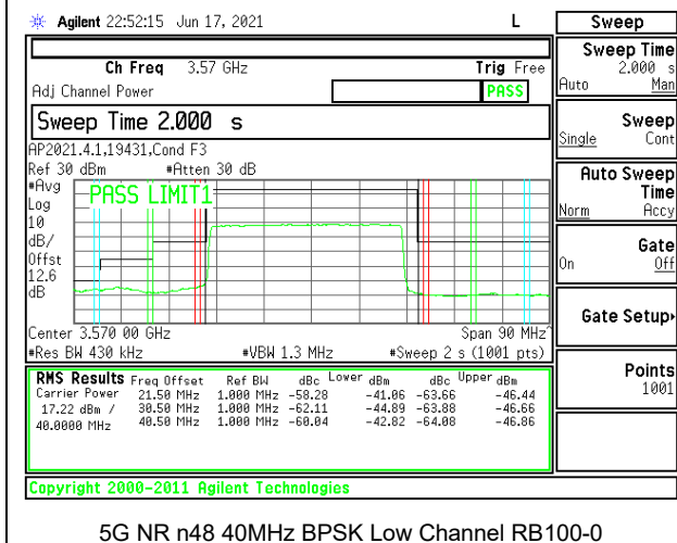
5G NR n48 40MHz BPSK Low Channel RB100-0
