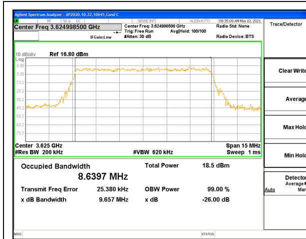
5G NR n48 10MHz BPSK Middle Channel RB23-0
