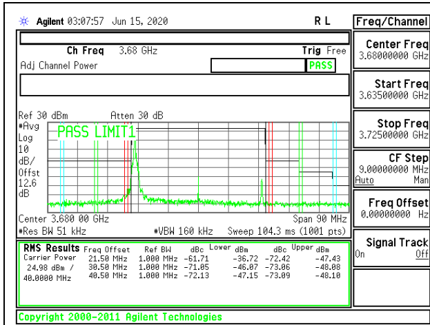
5G NR n48 40MHz BPSK High Channel RB1-0, ID:19431
