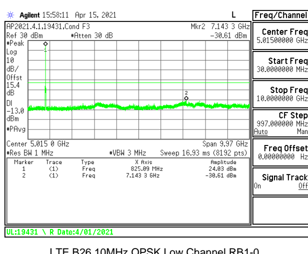
LTE B26 10MHz QPSK Low Channel RB1-0
