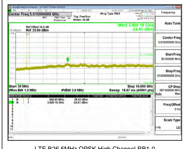
LTE B26 5MHz QPSK High Channel RB1-0
