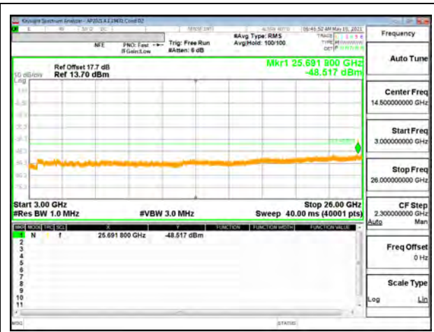
LTE B30 10MHz BPSK Middle Channel RB1-0 (3G to 26G)
