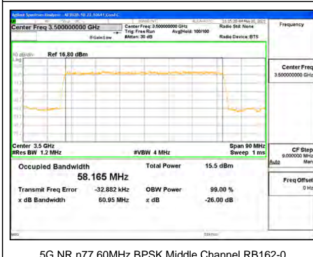
5G NR n77 60MHz BPSK Middle Channel RB162-0
