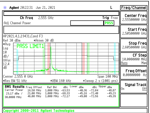
5G NR n7 30MHz BPSK High Channel RB1-0
