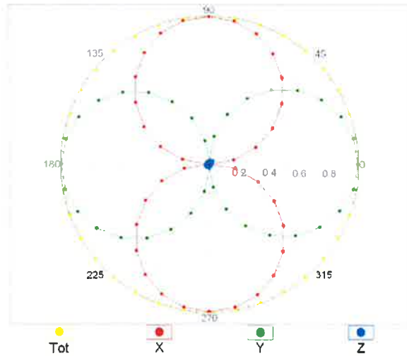
f=1800 MHz,R22,0°
