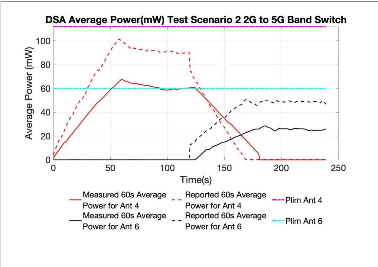
Figure 8 60 Second Average Power vs Time during Band Switch
