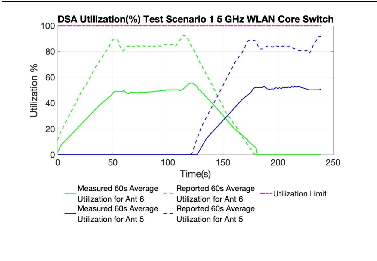
Figure 4 60 Second Aggregated SAR Utilization vs Time, 5GHz
