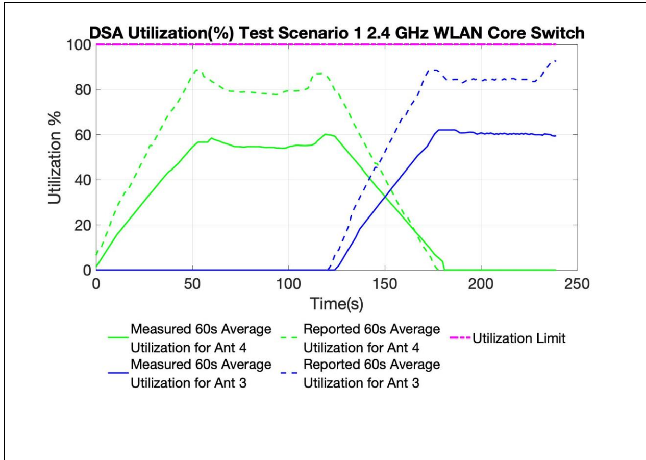
Figure 1 60 Second Aggregated SAR Utilization vs Time, 2.4GHz
