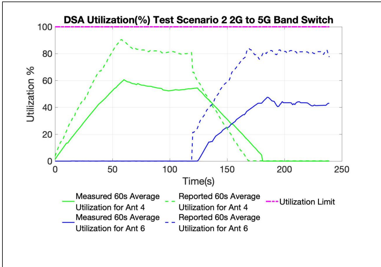
Figure 7 60 Second Aggregated SAR Utilization vs Time during Band Switch
