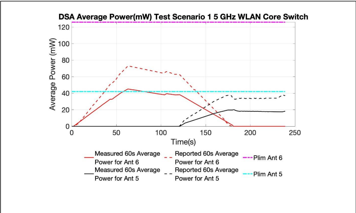
Figure 5 60 Second Average Power vs Time, 5GHz
