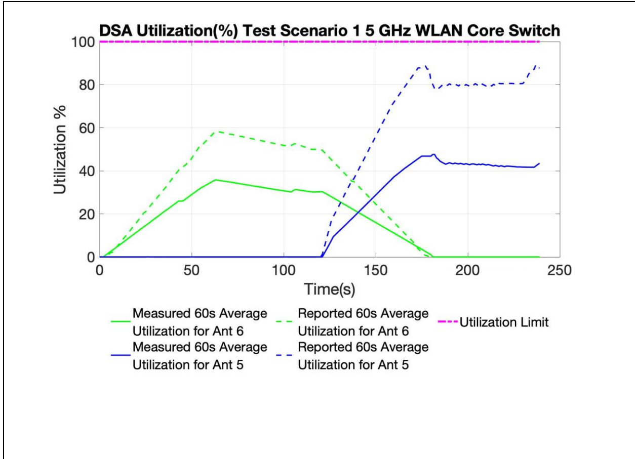
Figure 4 60 Second Aggregated SAR Utilization vs Time, 5GHz
