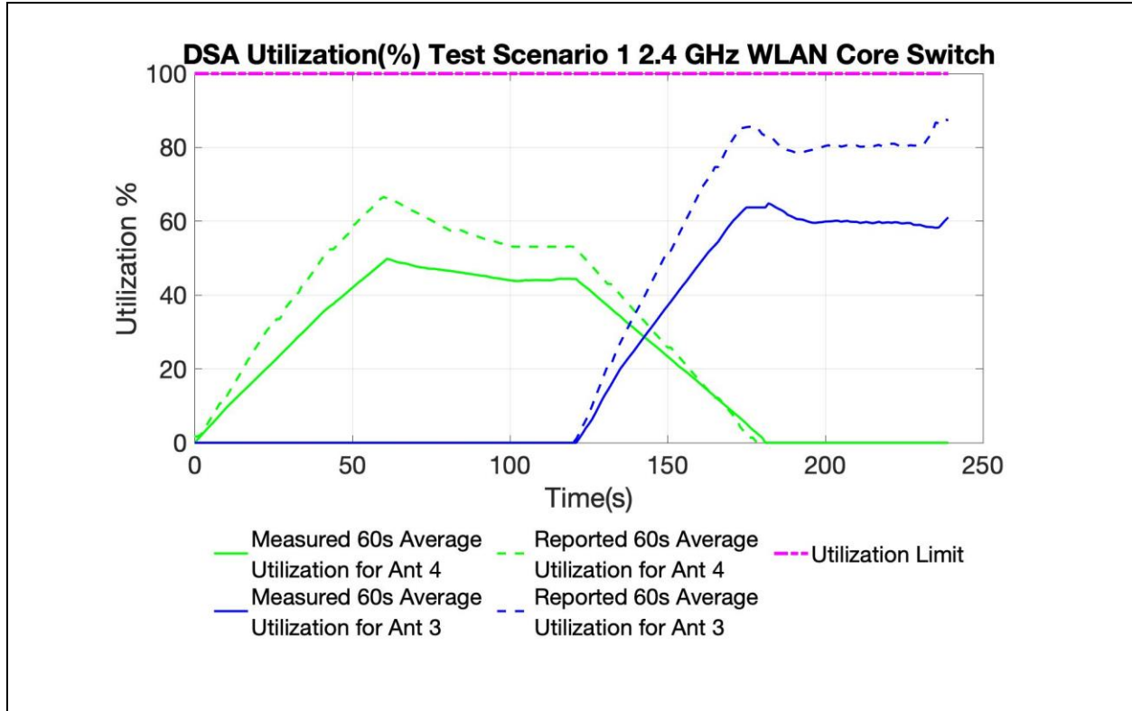
Figure 1 60 Second Aggregated SAR Utilization vs Time, 2.4GHz
