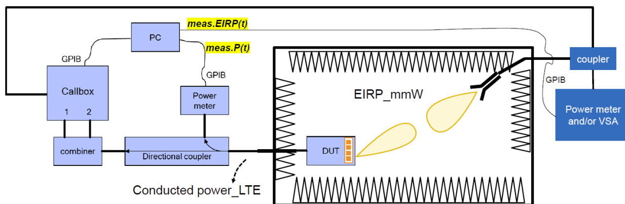
Figure 8-1: mmW NR radiated power measurement setup (see Appendix E for missing figures)
