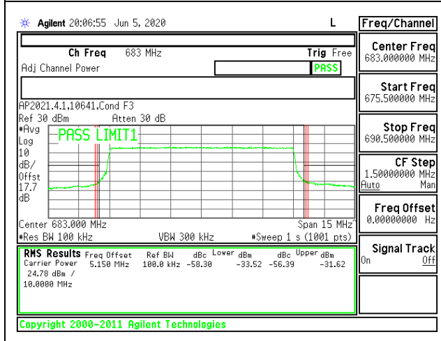
LTE B71 10MHz QPSK Middle Channel RB50-0
