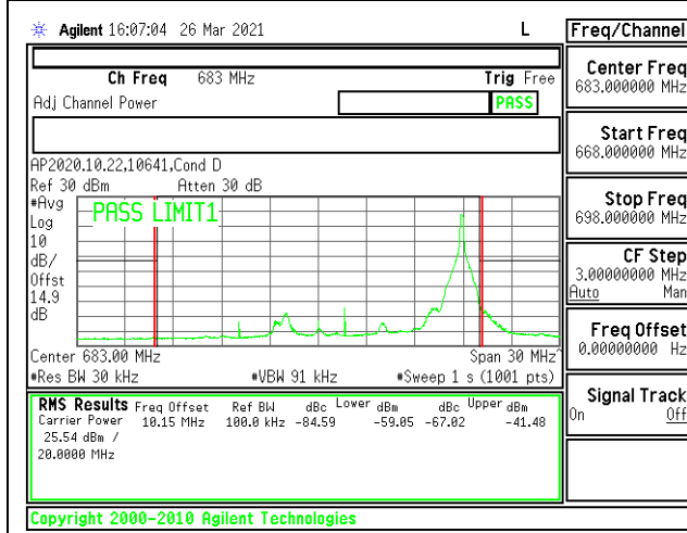
LTE B71 20MHz QPSK Middle Channel RB1-99
