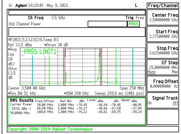
5G NR n77 70MHz BPSK Middle Channel RB1-187
