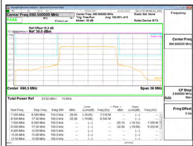
LTE B71 15MHz QPSK High Channel RB75-0
