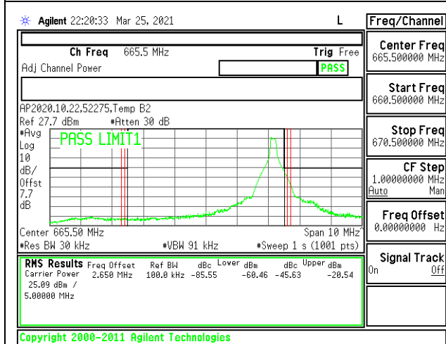
5G NR n71 5MHz BPSK Low Channel RB1-24
