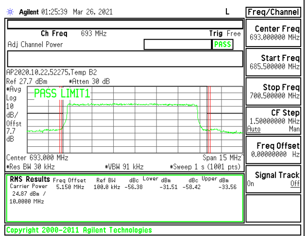
5G NR n71 10MHz BPSK High Channel RB50-0
