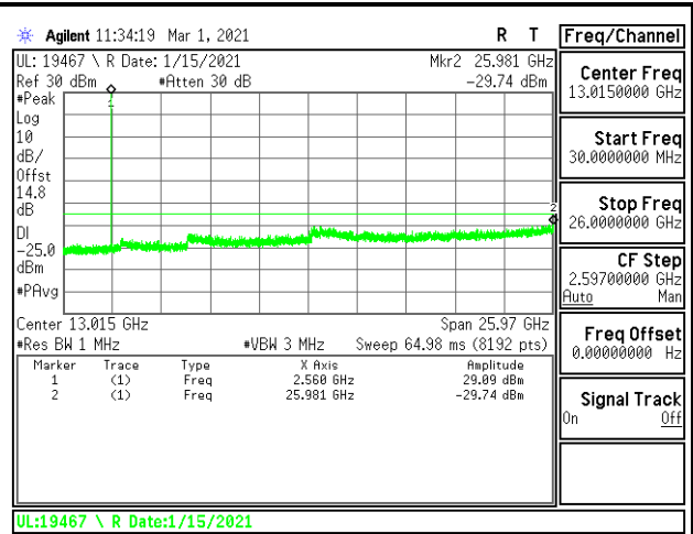
LTE B7 10MHz QPSK High Channel RB1-0
