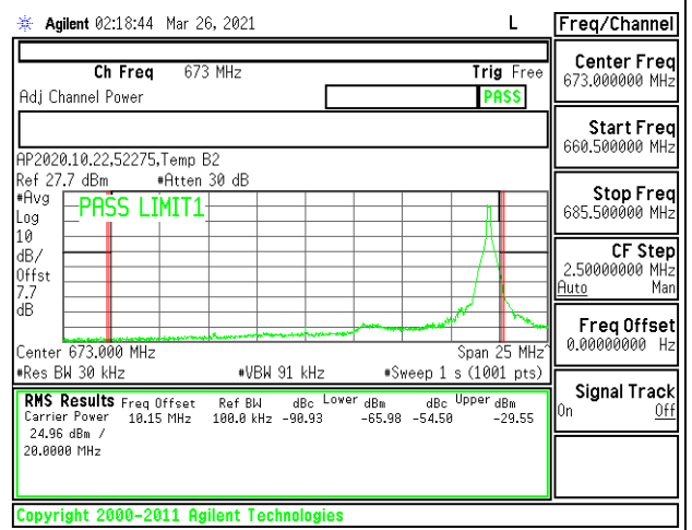
5G NR n71 20MHz BPSK Low Channel RB1-105
