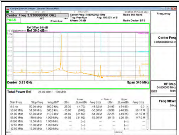
5G NR n77 100MHz BPSK High Channel RB1-0
