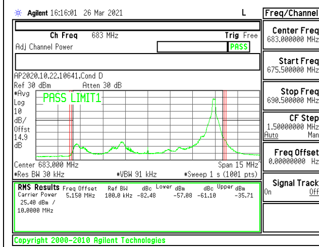
LTE B71 10MHz QPSK Middle Channel RB1-49
