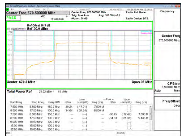
LTE B71 15MHz QPSK Low Channel RB75-0
