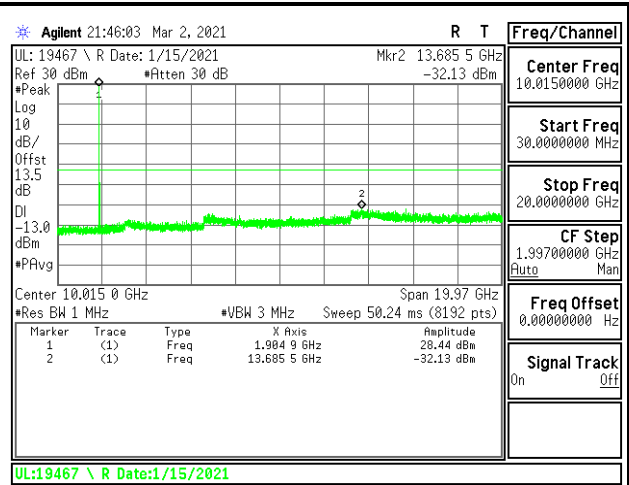
LTE B25 10MHz QPSK High Channel RB1-0
