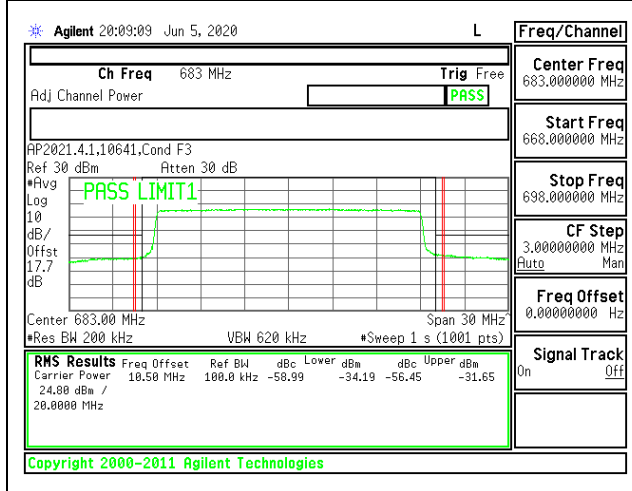
LTE B71 20MHz QPSK Middle Channel RB100-0
