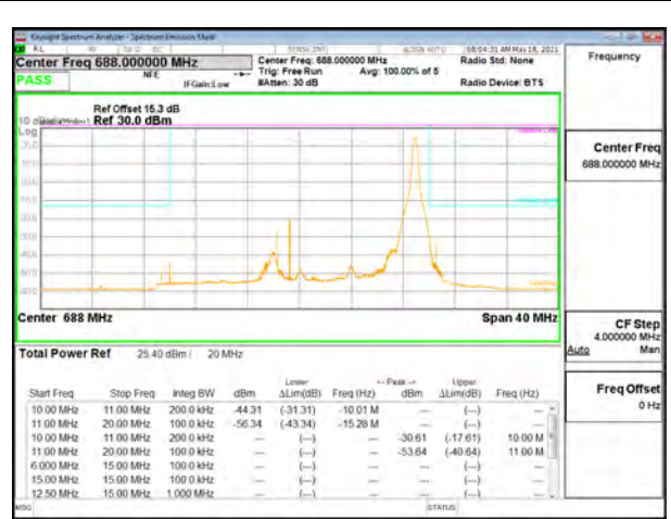
LTE B71 20MHz QPSK High Channel RB1-99
