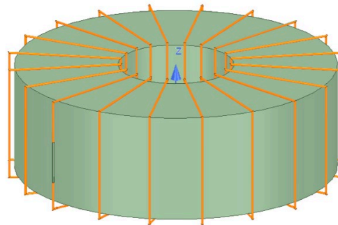
Figure 3: Toroid Model
