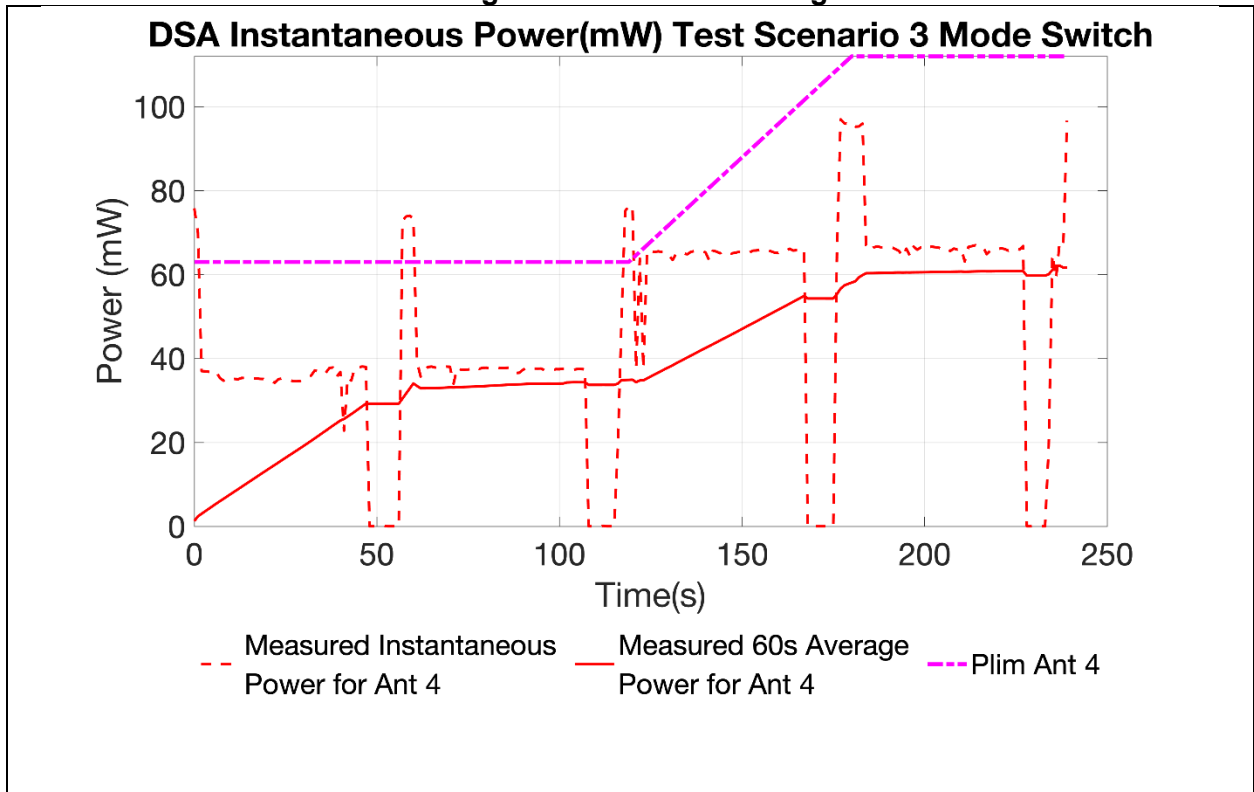
Figure 12 60 Second Average Power vs Time during Mode Switch and Instantaneous Power
