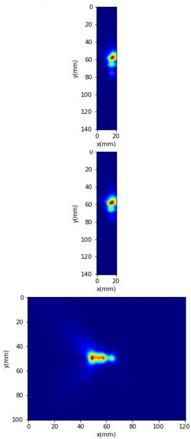
Power Density Plots for Beam ID: 132
