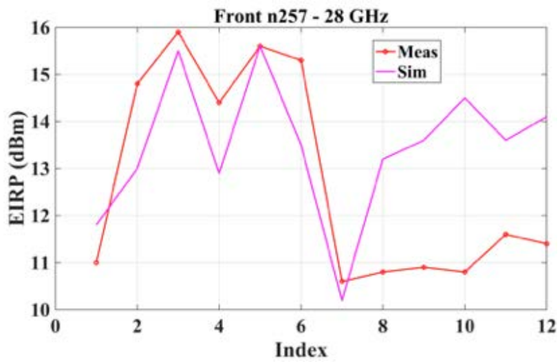
Figure 11. Simulated vs. Measured EIRP at 28 GHz for (a) side-firing antenna, (b) back-firing antenna, (c) front-firing antenna.
