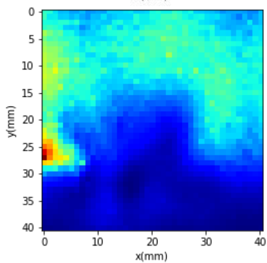
Power Density Plots for Beam ID:20
