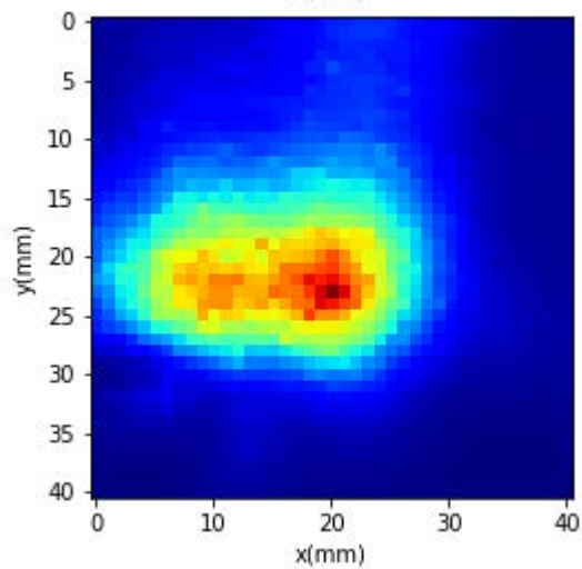
Power Density Plots for Beam ID:158
