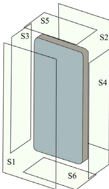
Figure 5. Evaluating surfaces for MPE (PD).
