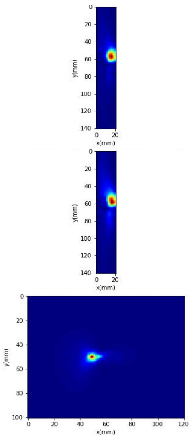
Power Density Plots for Beam ID: 148
