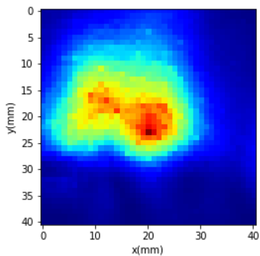
Power Density Plots for Beam ID:146
