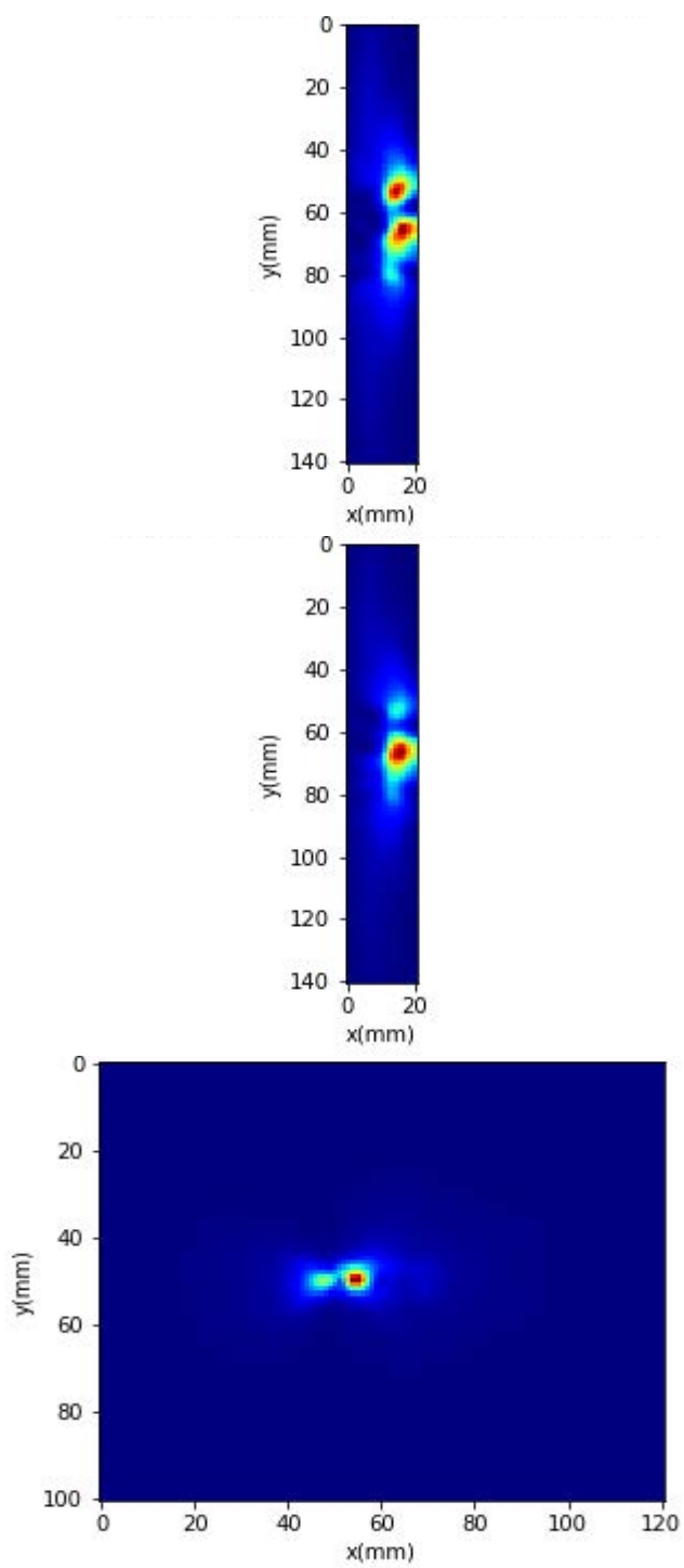
Power Density Plots for Beam ID: 154
