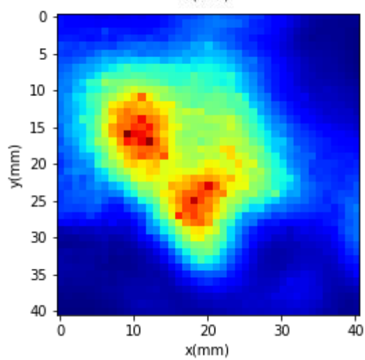
Power Density Plots for Beam ID:159
