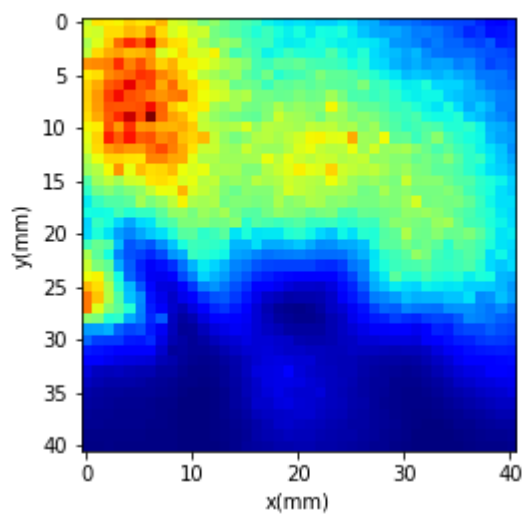
Power Density Plots for Beam ID:18
