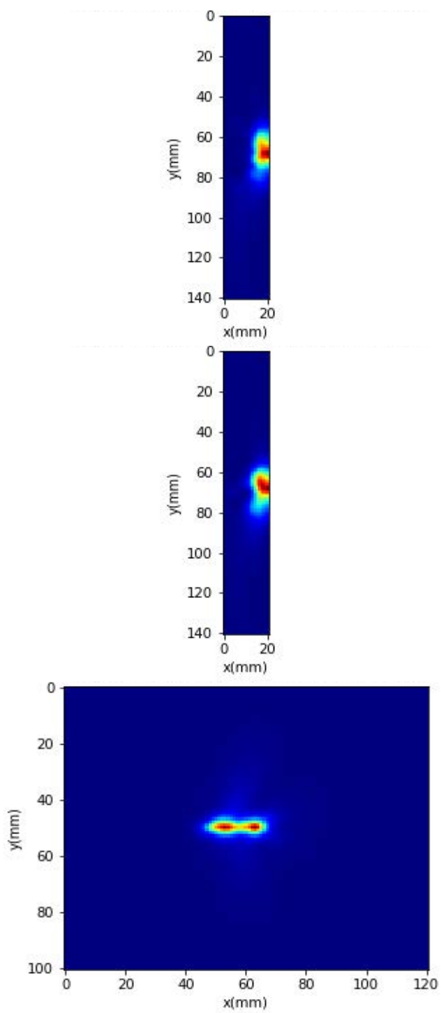
Power Density Plots for Beam ID: 157
