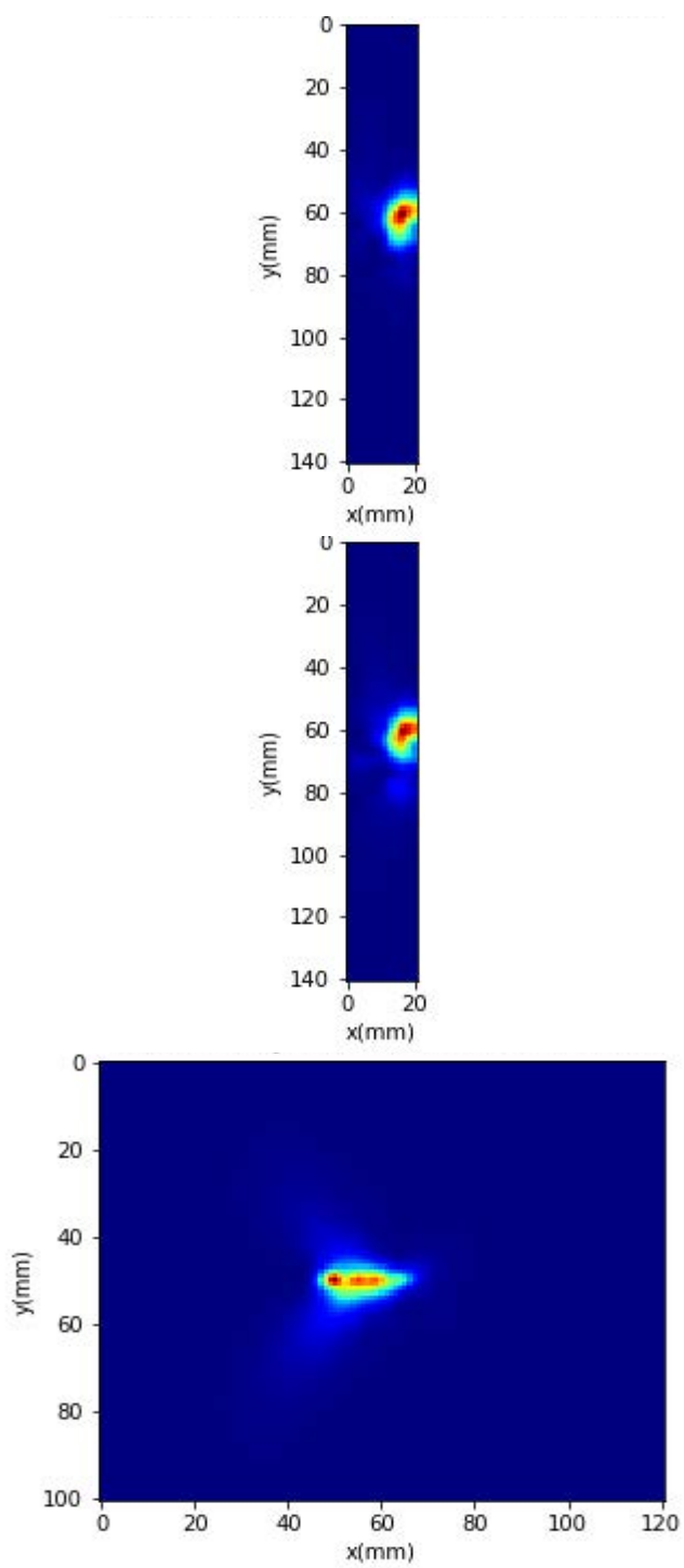
Power Density Plots for Beam ID: 156
