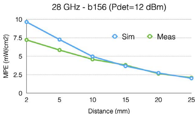
Figure 13. Simulation and measurement comparison with increasing distance from DUT.
