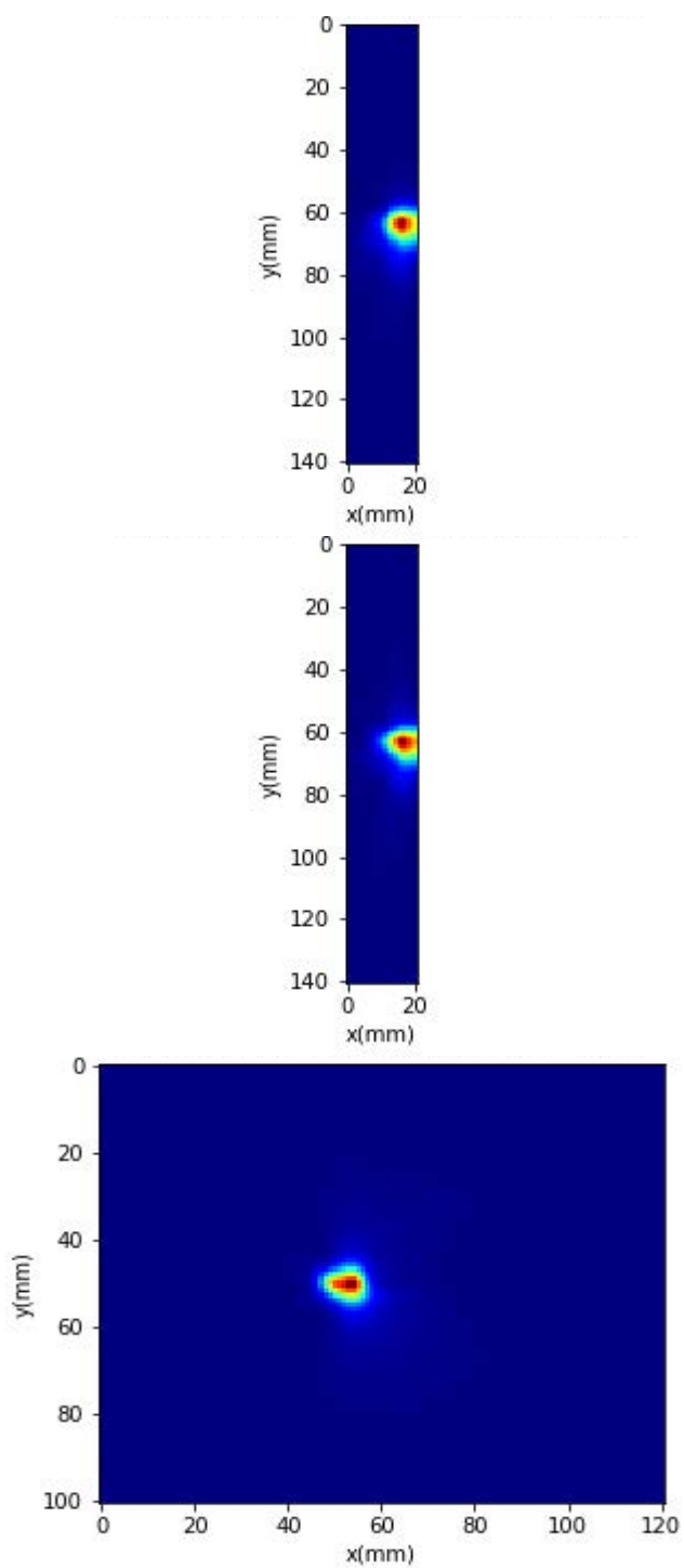
Power Density Plots for Beam ID: 20
