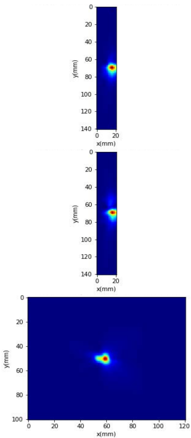
Power Density Plots for Beam ID: 13
