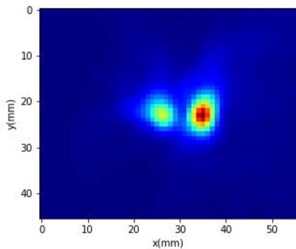
Power Density Plots for Beam ID:149
