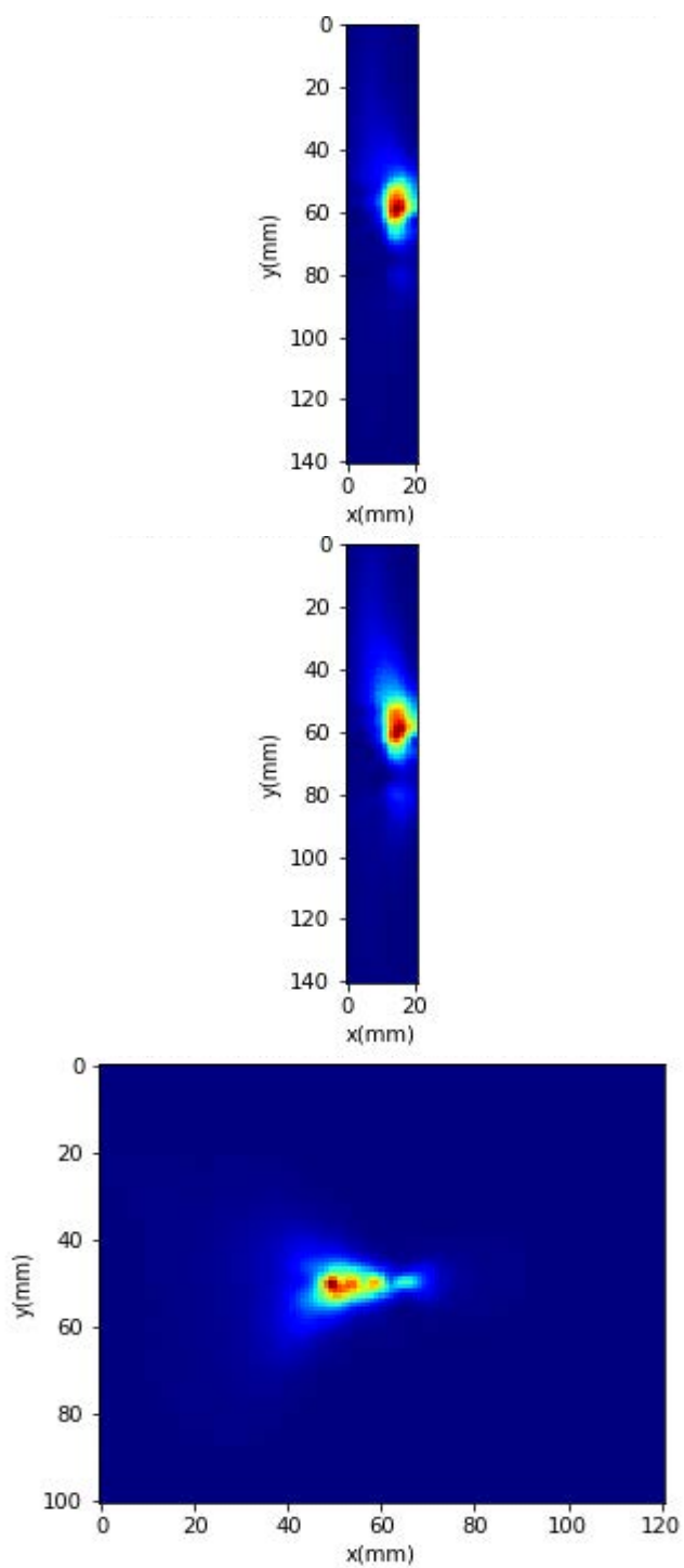
Power Density Plots for Beam ID: 164
