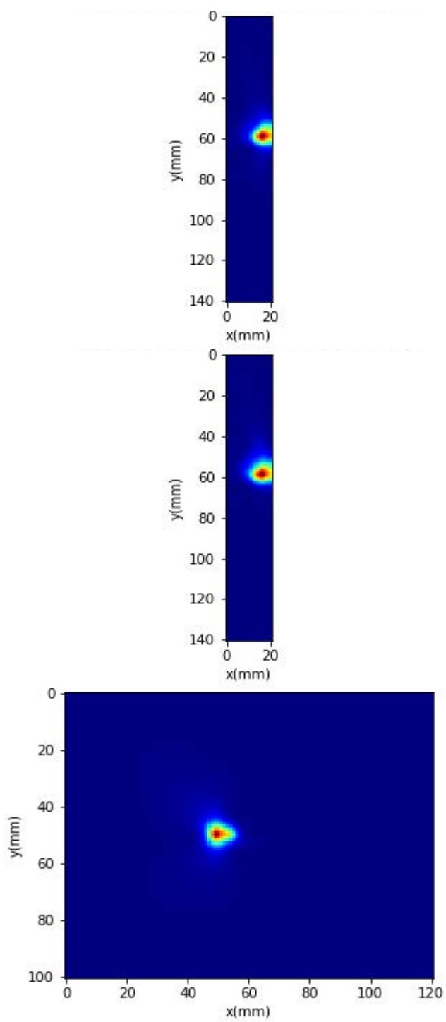
Power Density Plots for Beam ID: 26
