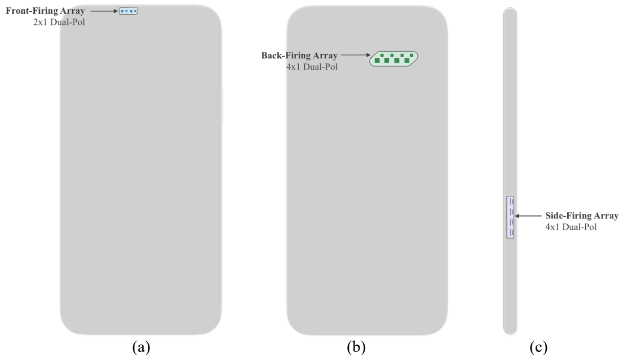
Figure 4. Schematic of the simulation model, which consists of three 5G antenna arrays, (a) front view, (b) rear view and (c) side view.
