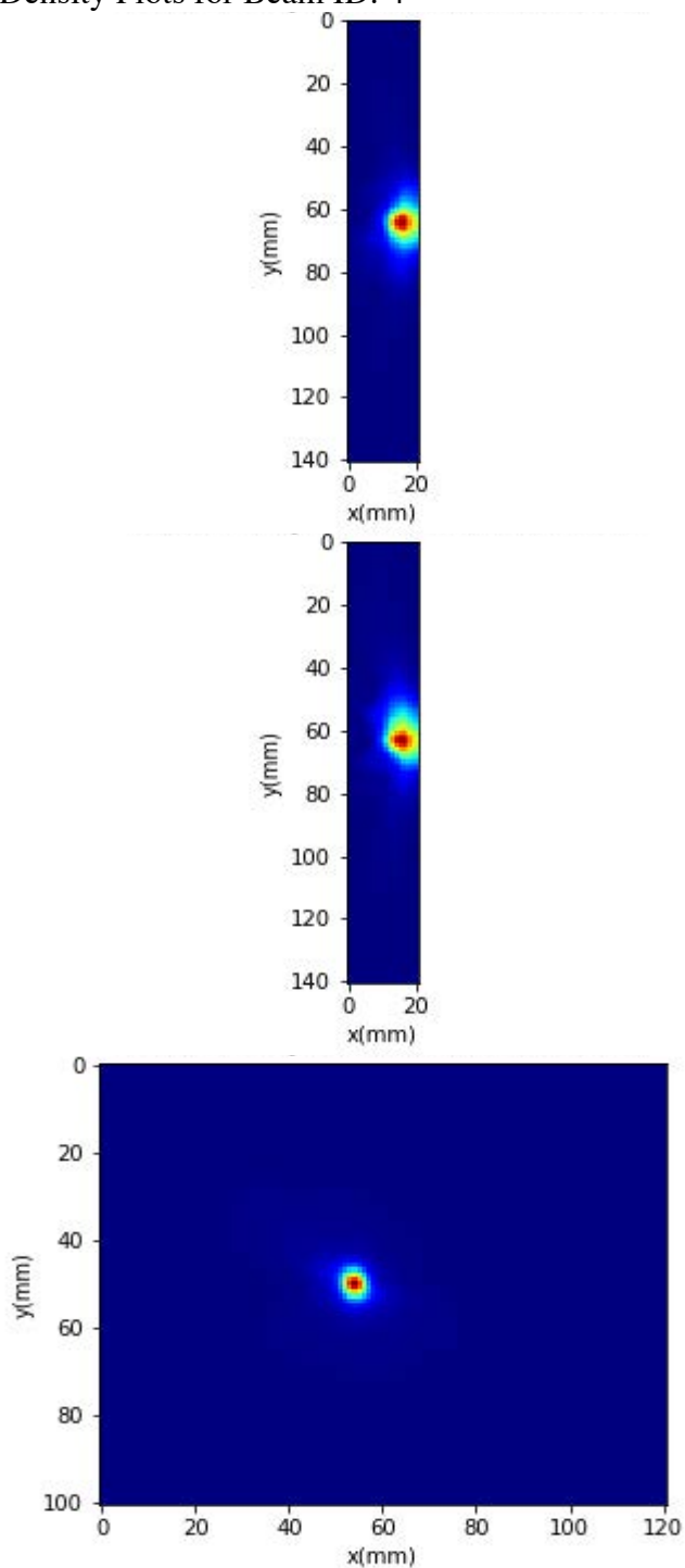
Power Density Plots for Beam ID: 4
