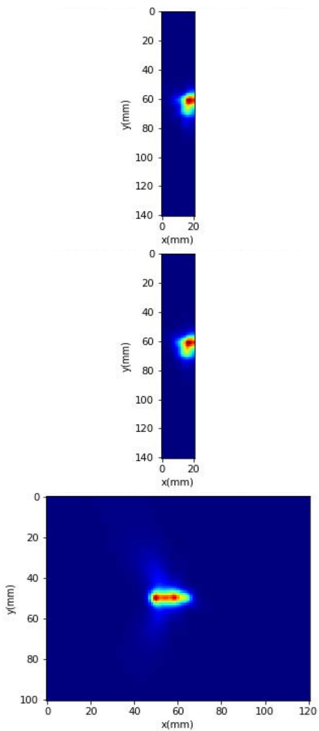
Power Density Plots for Beam ID: 38
