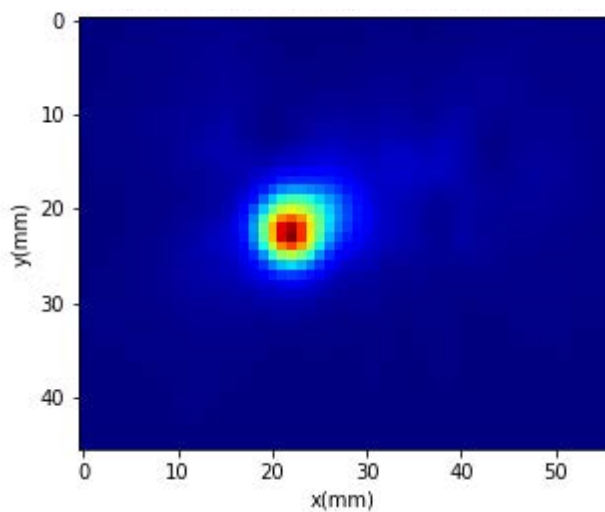
Power Density Plots for Beam ID:128
