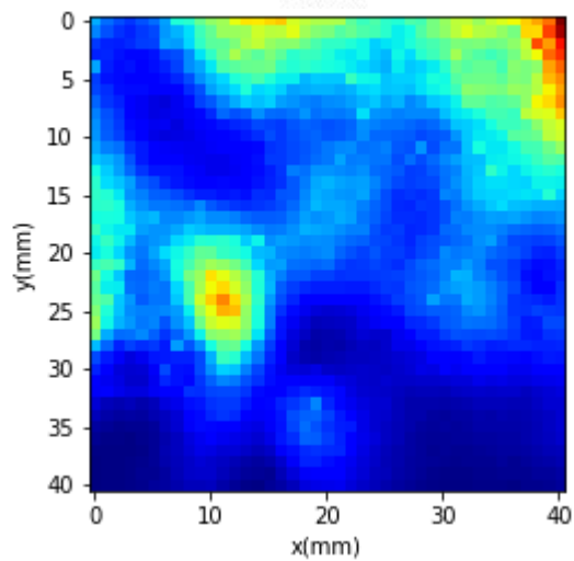
Power Density Plots for Beam ID:19
