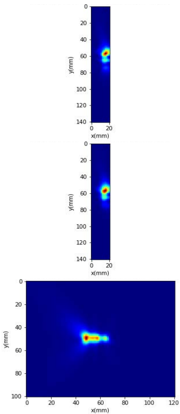
Power Density Plots for Beam ID: 35
