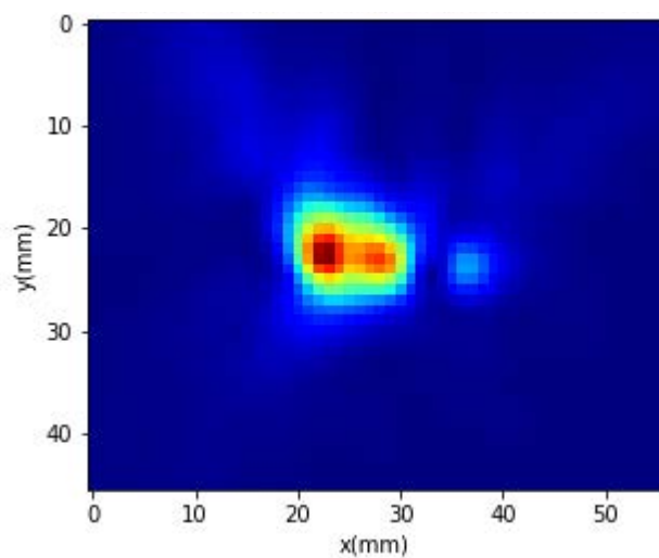
Power Density Plots for Beam ID:146
