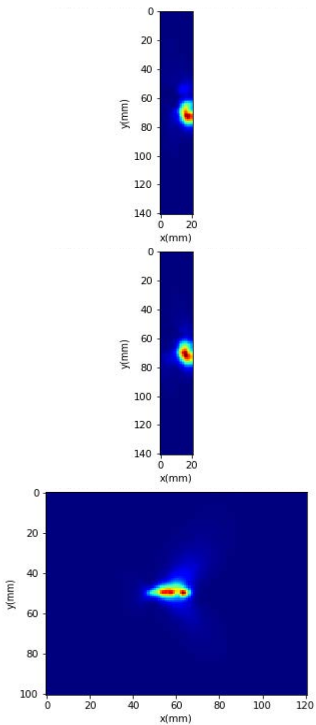
Power Density Plots for Beam ID: 166
