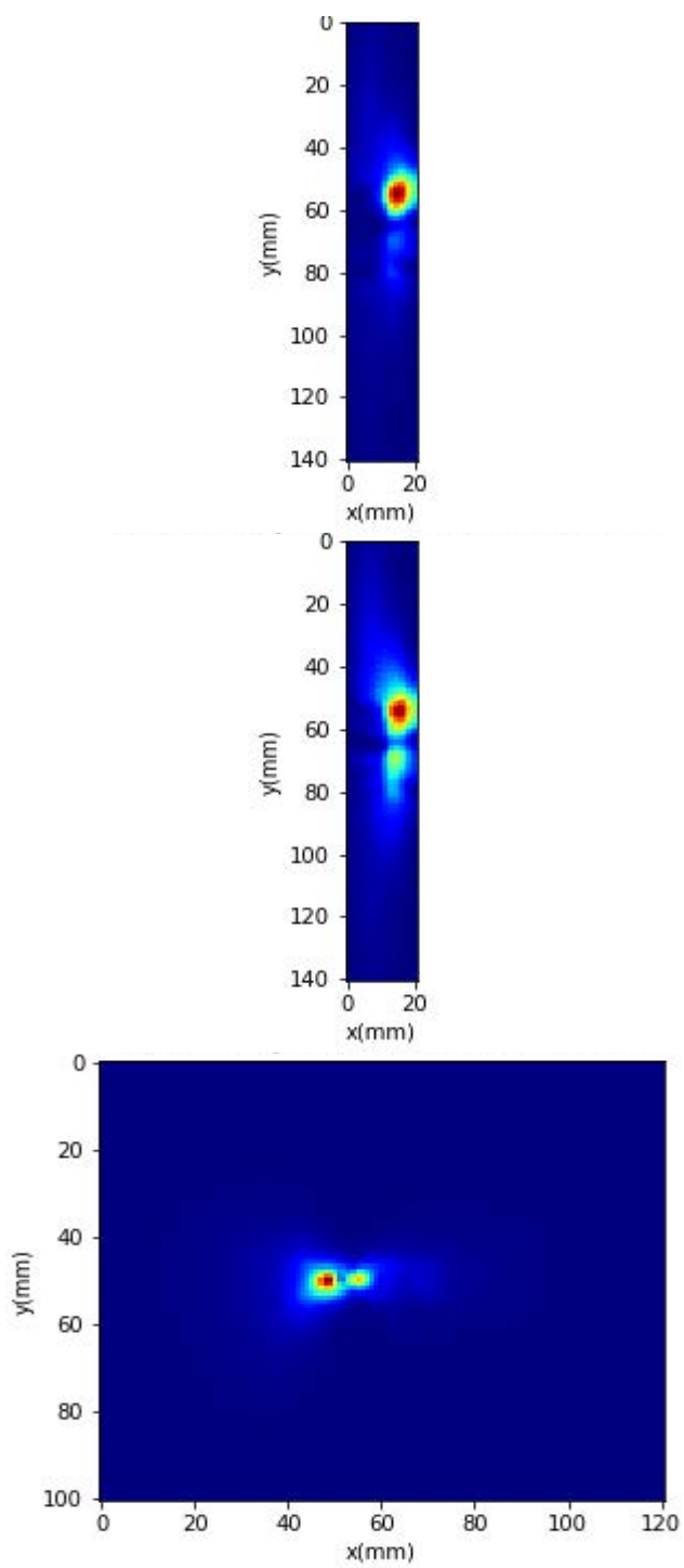
Power Density Plots for Beam ID: 141
