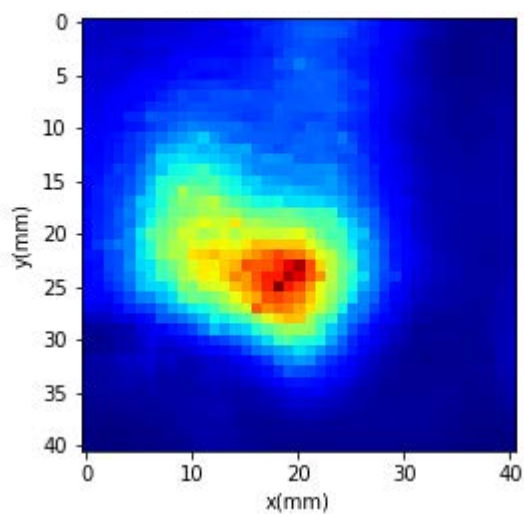
Power Density Plots for Beam ID:149
