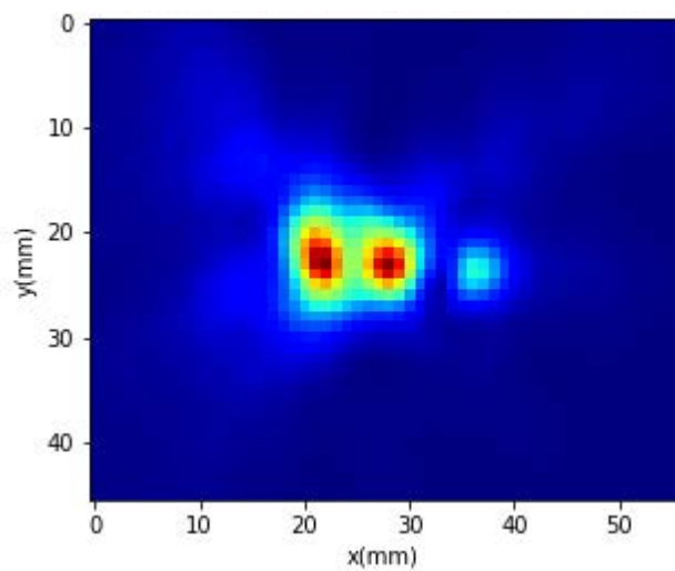
Power Density Plots for Beam ID:156
