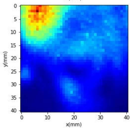
Power Density Plots for Beam ID:28
