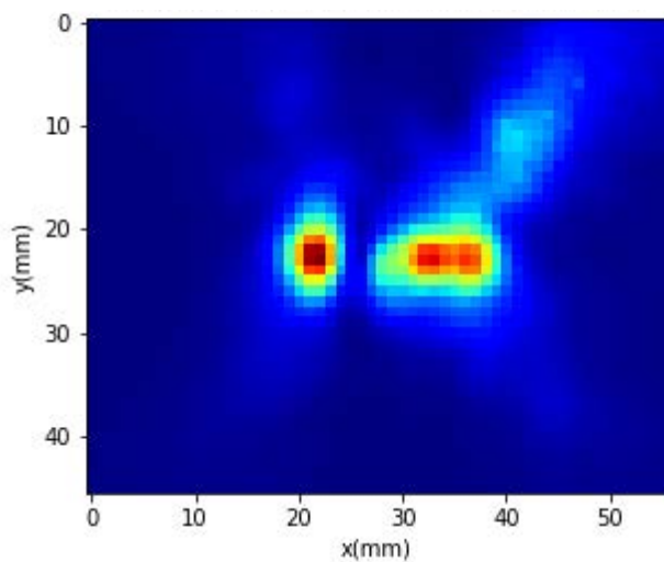
Power Density Plots for Beam ID:21
