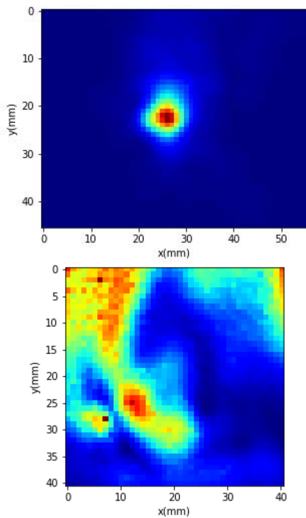
Power Density Plots for Beam ID:4
