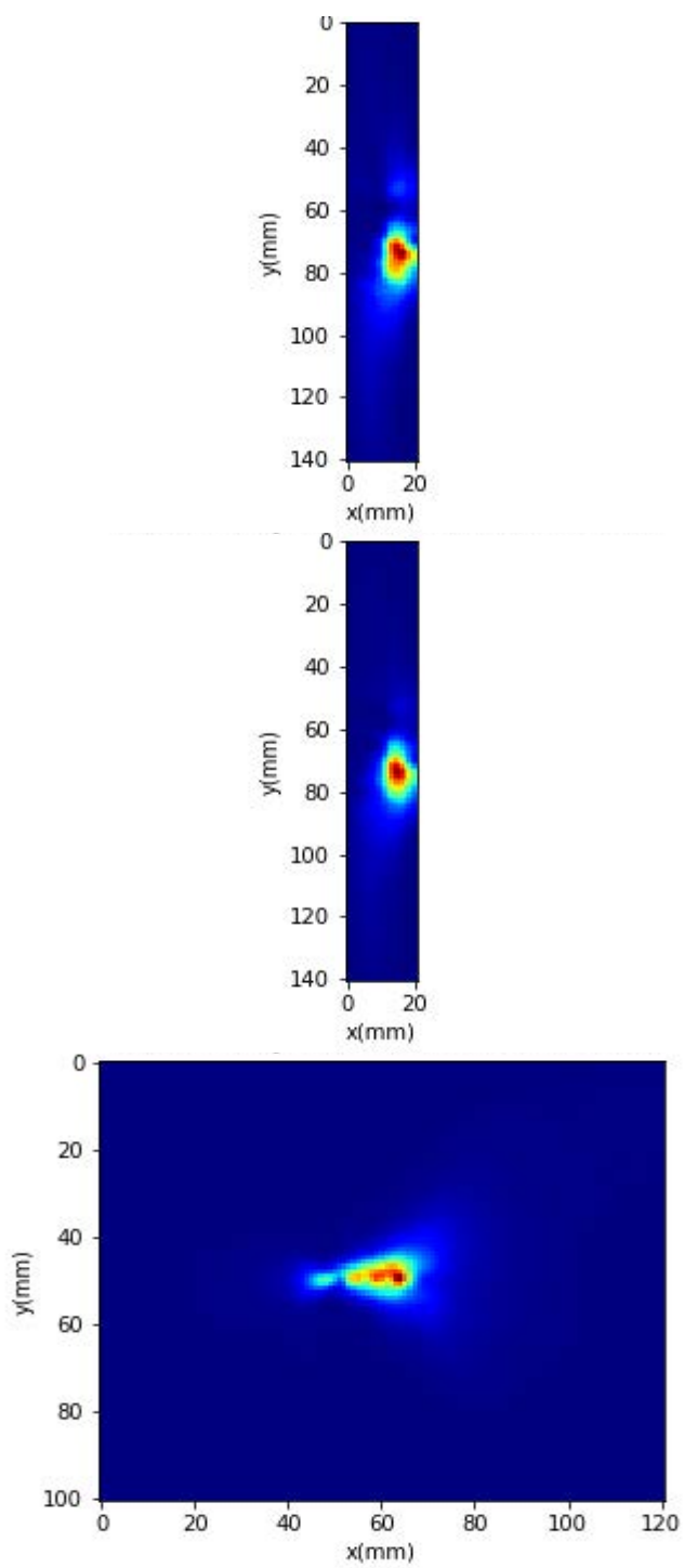
Power Density Plots for Beam ID: 158
