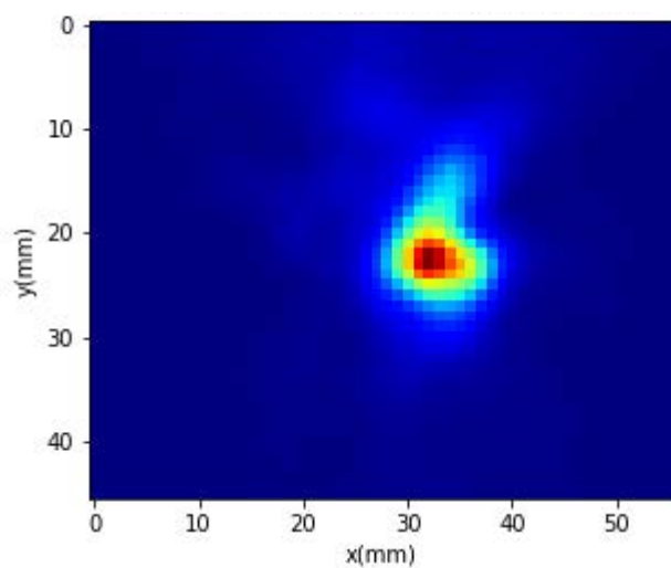
Power Density Plots for Beam ID:5
