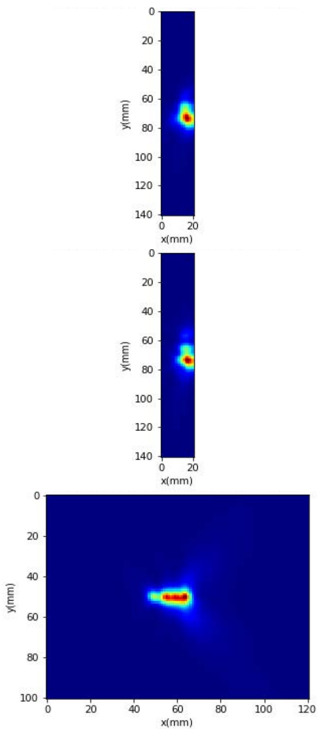
Power Density Plots for Beam ID: 27
