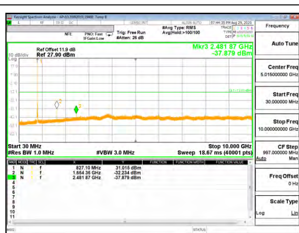
5G NR Bn5 20MHz QPSK Middle Channel RB1-0
