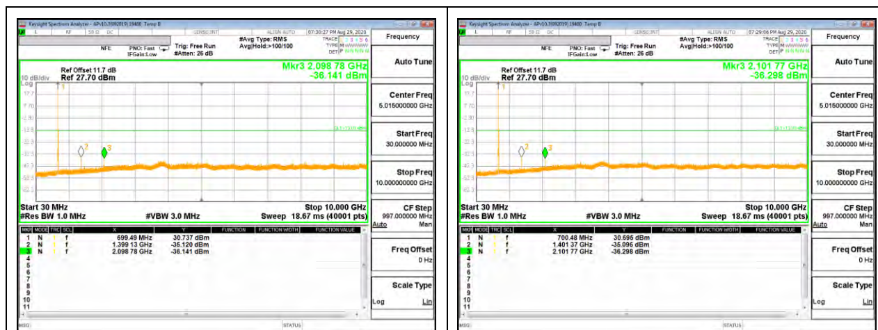
5G NR Bn12 15MHz QPSK Low Channel RB1-0
