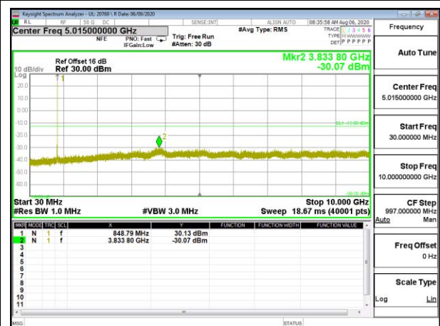
CDMA BC0 1xEV-DO Rev A High Channel
