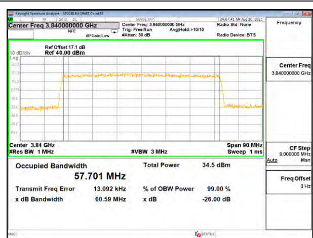
5G NR Band n77 60MHz QPSK Middle Channel RB162-0
