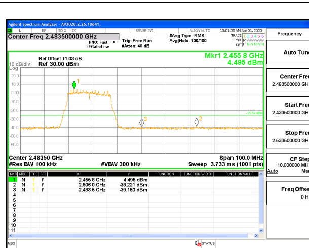
HIGH CHANNEL 11 BANDEDGE ANT 4
