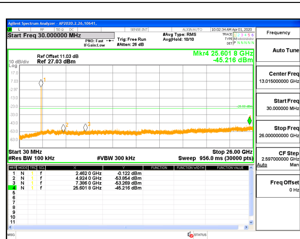
OUT-OF-BAND HIGH CHANNEL 11 ANT 4
