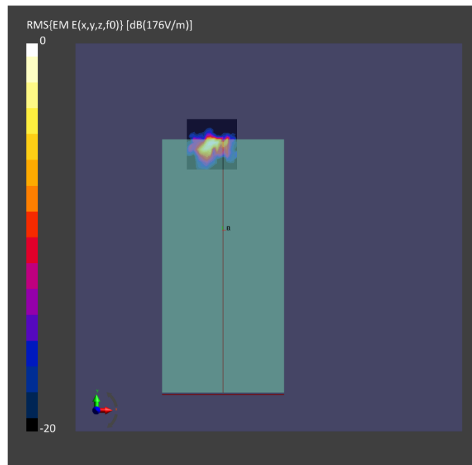
Figure 4-1: Band 260, beam ID 6/134, 4cm 2 PD, Front
