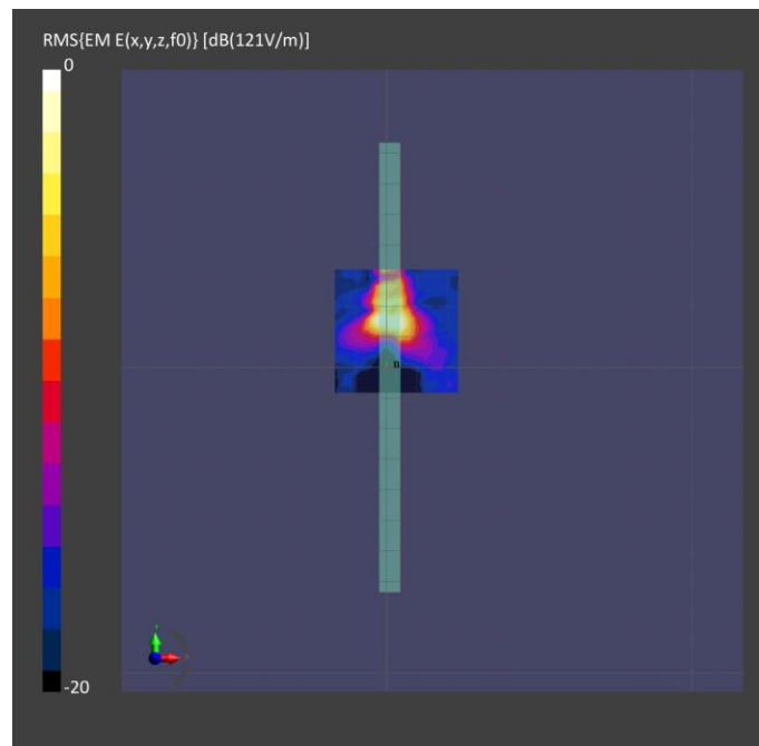
Figure 4-2: Band 261, beam ID 27, 4cm 2 PD, Edge Right
