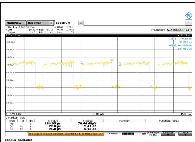
DUTY CYCLE 802.11ac VHT80 1TX MODE MCS9
