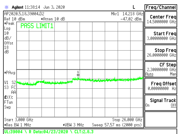
LTE B30 10MHz QPSK Mid Channel RB1-0 (3G to 26G)
