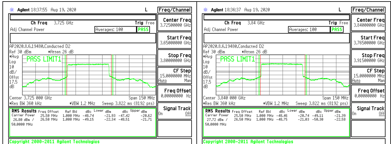
5G NR Band n77 50MHz QPSK Low Channel RB128-0
