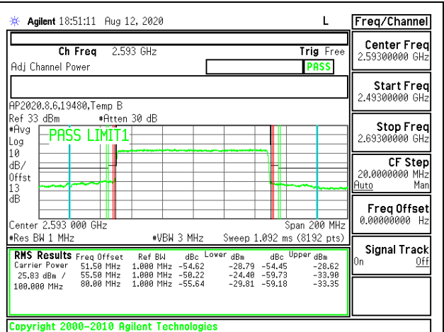
5G NR Band n41 100MHz QPSK Middle Channel RB270-0
