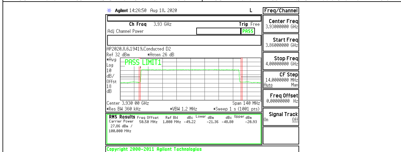
5G NR Band n77 100MHz QPSK High Channel RB270-0
