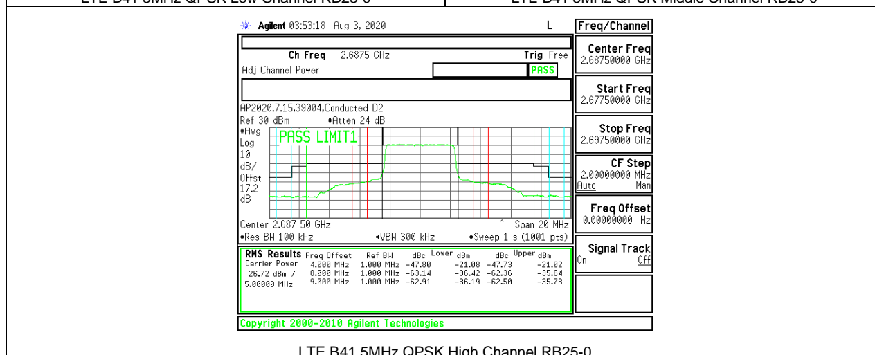
LTE B41 5MHz QPSK High Channel RB25-0
