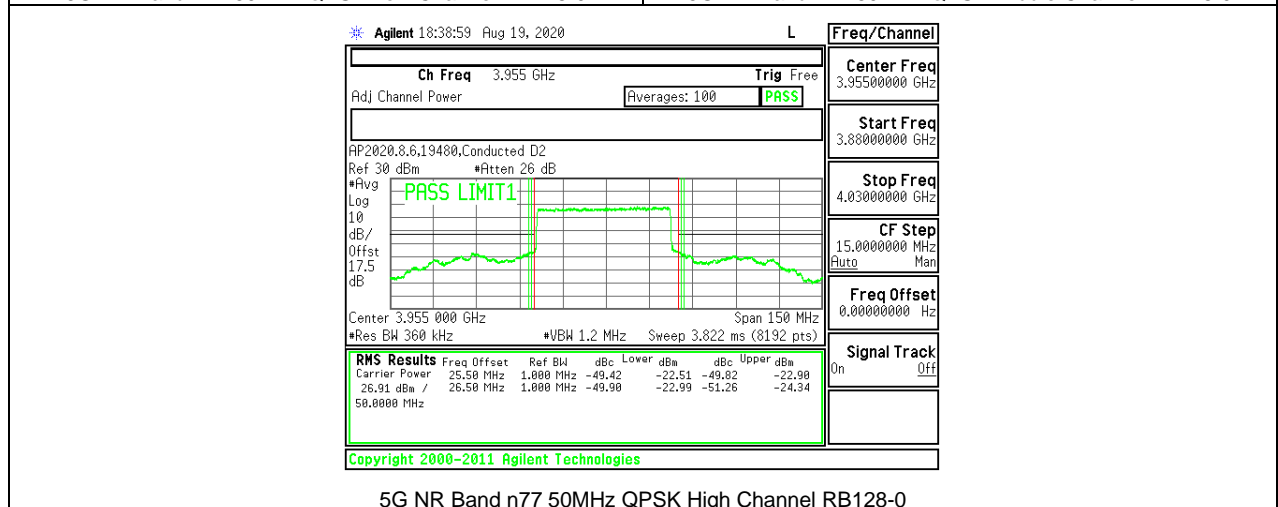
5G NR Band n77 50MHz QPSK High Channel RB128-0
