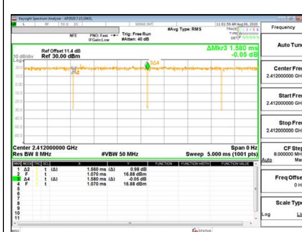
DUTY CYCLE 802.11ax HE20 MCS9
