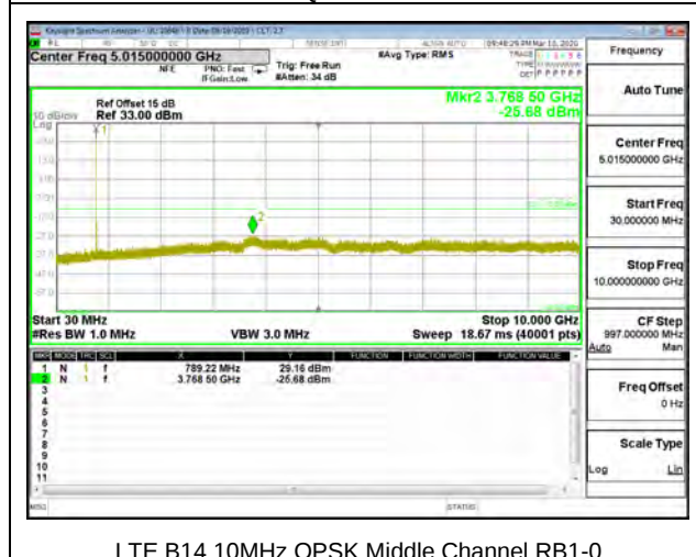
LTE B14 10MHz QPSK Middle Channel RB1-0
