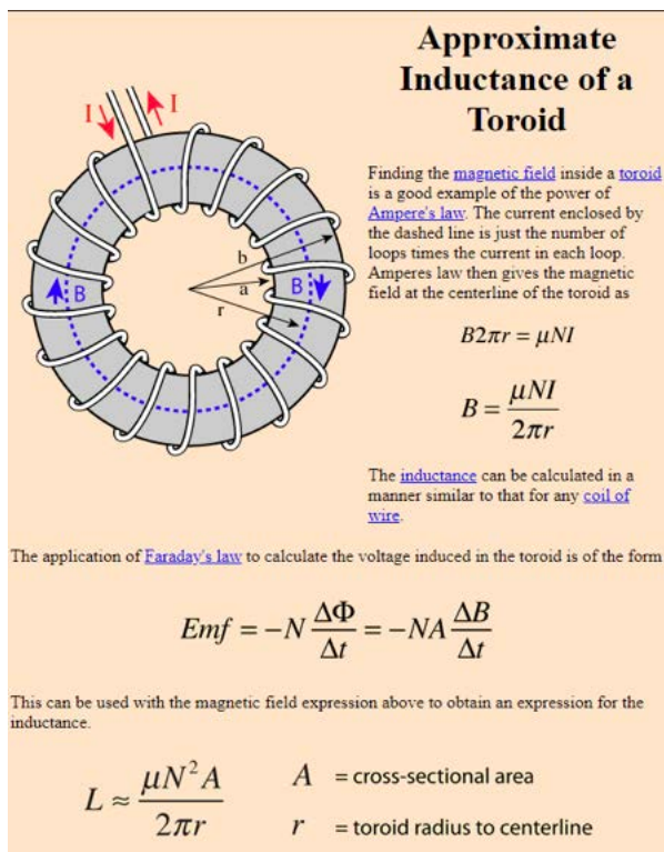
Figure 3: Toroid Model
