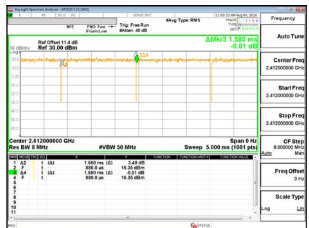
DUTY CYCLE 802.11ax HE20 MCS0
