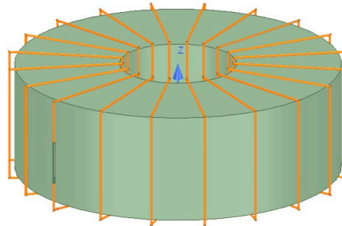
Figure 3: Toroid Model
