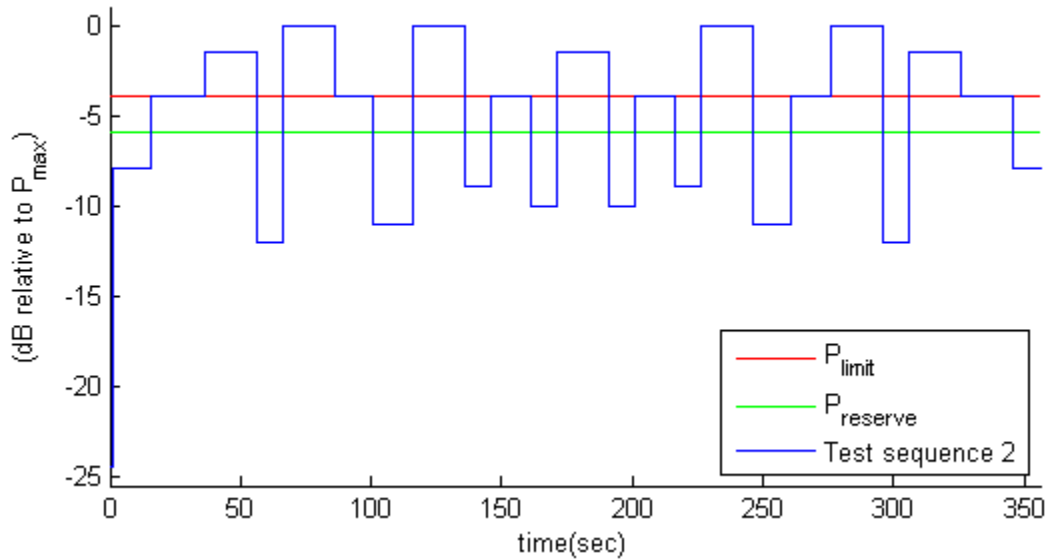
Figure A-2 Test sequence 2 waveform
