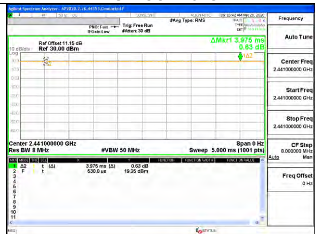
BLUETOOTH 8PSK
