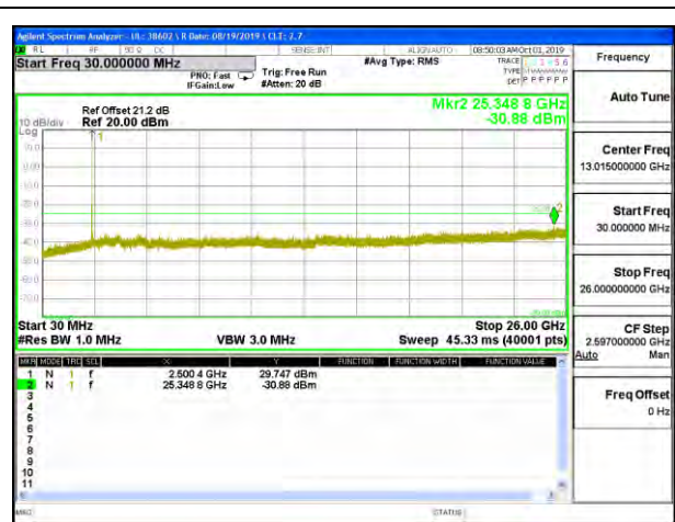
LTE B7 10MHz 16QAM Low Channel RB1-0
