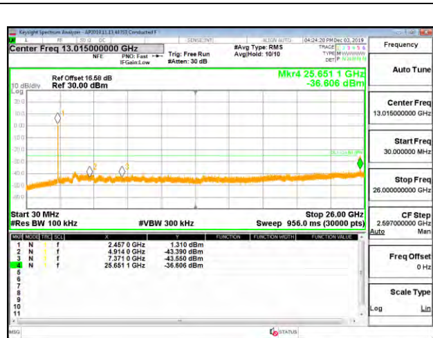
OUT-OF-BAND HIGH CHANNEL 10 LAT 3
