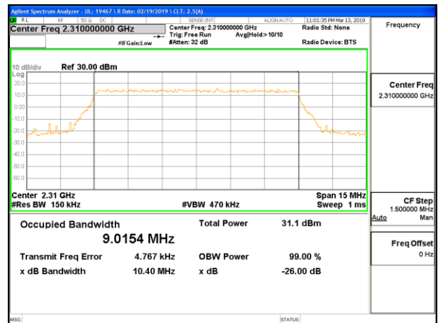
LTE B30 10MHz 64QAM Middle Channel RB50-0
