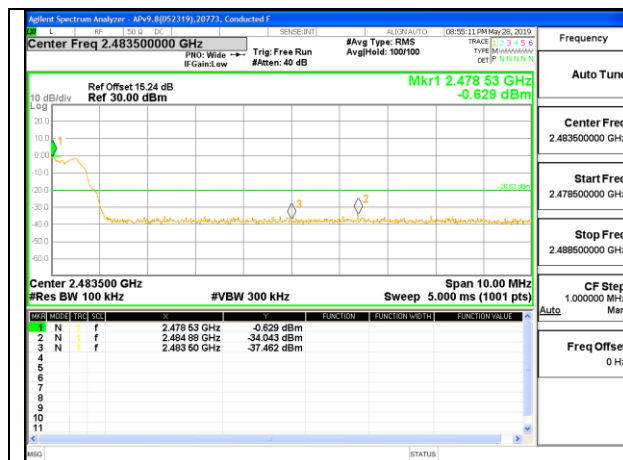
HIGH CHANNEL BANDEDGE ANT 5
