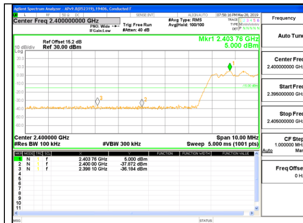
LOW CHANNEL , BANDEDGE ANT 5
