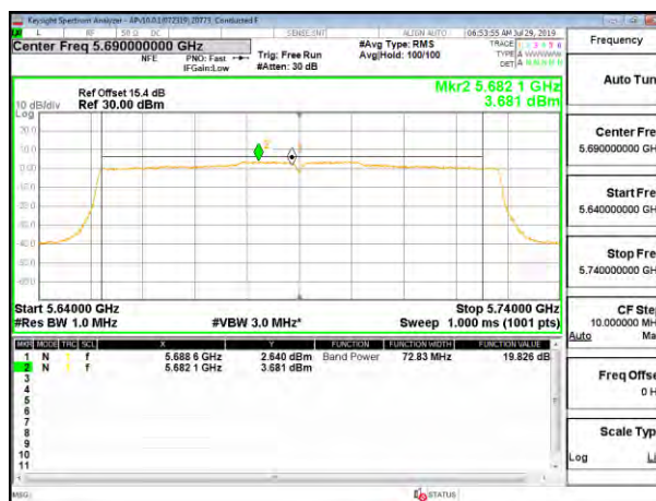
CHANNEL 138 ANTENNA 5
