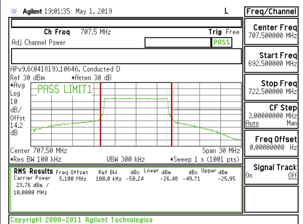
LTE B12 10MHz 16QAM Mid Channel RB50-0
