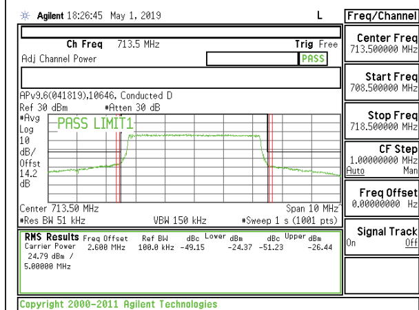
LTE B12 5MHz QPSK High Channel RB25-0
