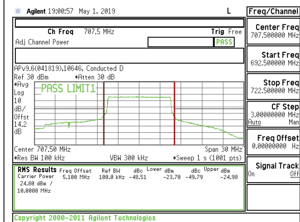
LTE B12 10MHz QPSK Mid Channel RB50-0
