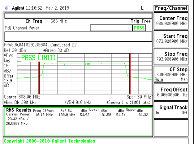
LTE B71 20MHz 16QAM High Channel RB100-0
