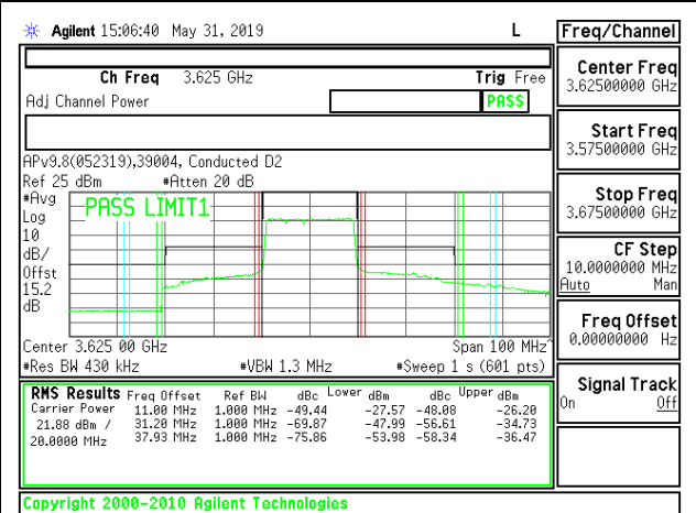
LTE B48 20MHz 16QAM Mid Channel RB100-0
