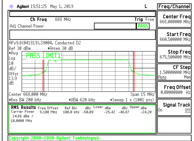
LTE B71 10MHz QPSK Low Channel RB50-0
