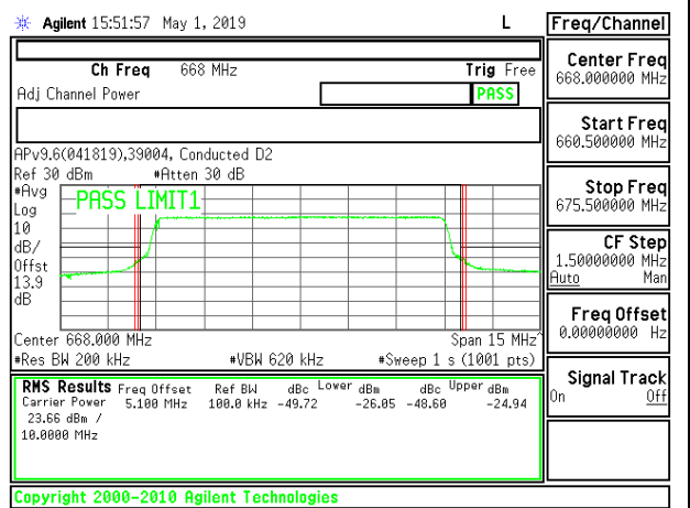
LTE B71 10MHz 16QAM Low Channel RB50-0
