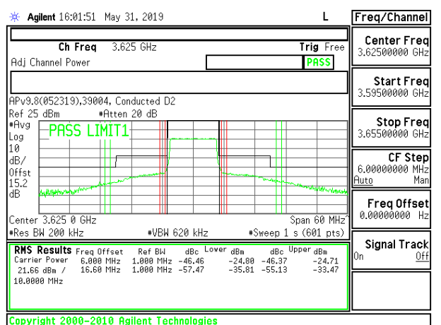
LTE B48 10MHz 16QAM Mid Channel RB50-0
