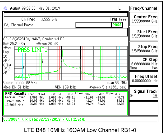
LTE B48 10MHz 16QAM Low Channel RB1-0
