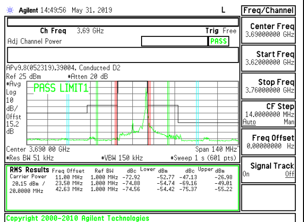
LTE B48 20MHz 16QAM High Channel RB1-99
