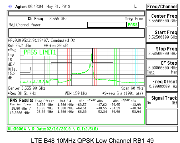
LTE B48 10MHz QPSK Low Channel RB1-49
