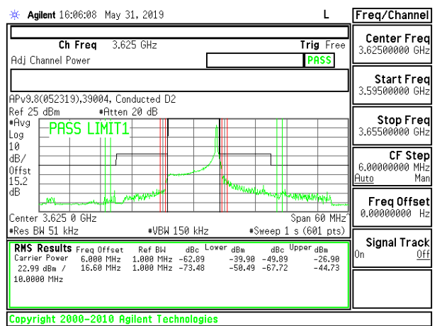
LTE B48 10MHz 16QAM Mid Channel RB1-49
