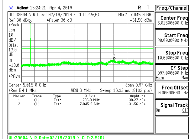
LTE B17 10MHz QPSK High Channel RB1-0
