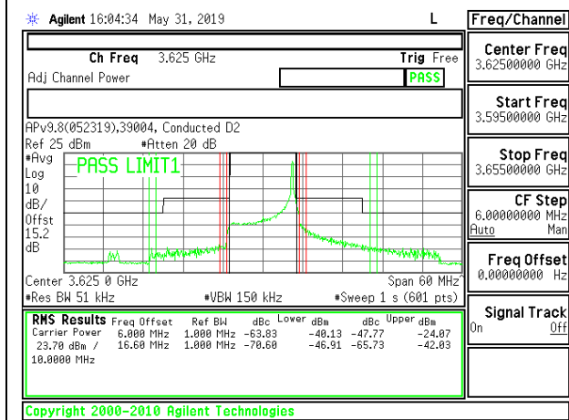
LTE B48 10MHz QPSK Mid Channel RB1-49
