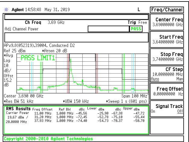
LTE B48 20MHz 16QAM High Channel RB1-0
