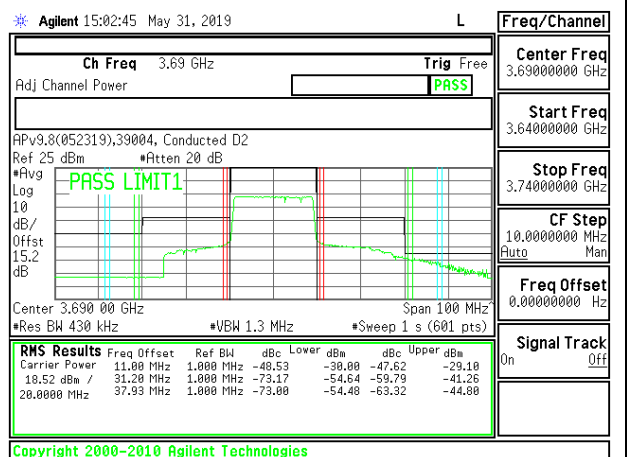
LTE B48 20MHz 16QAM High Channel RB100-0
