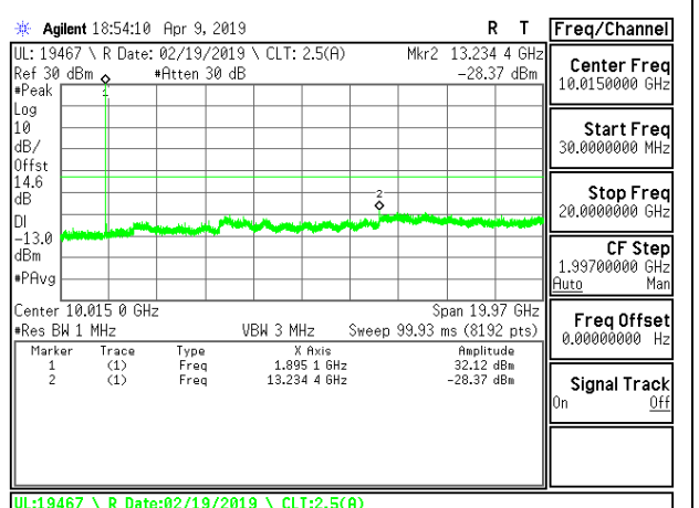
LTE B2 15MHz 16QAM High Channel RB1-0
