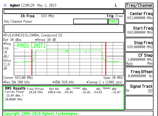
LTE B71 20MHz 16QAM Middle Channel RB100-0
