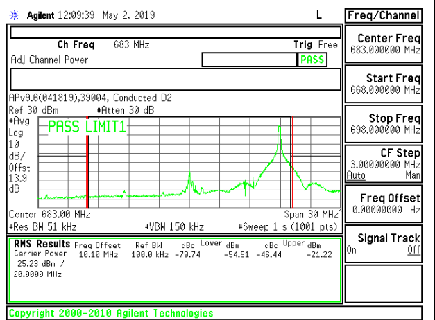
LTE B71 20MHz 16QAM Middle Channel RB1-99
