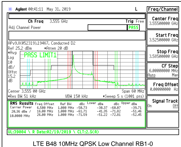
LTE B48 10MHz QPSK Low Channel RB1-0
