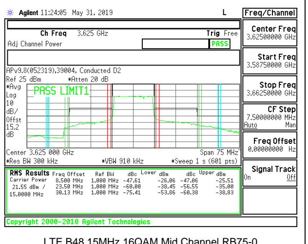
LTE B48 15MHz 16QAM Mid Channel RB75-0
