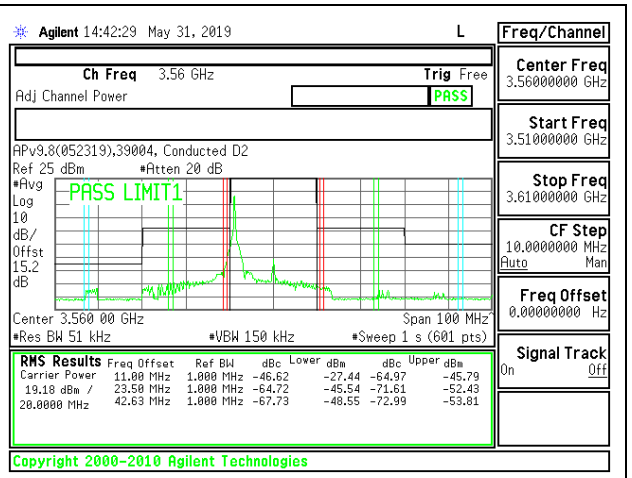
LTE B48 20MHz 16QAM Low Channel RB1-0
