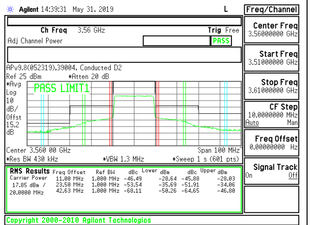
LTE B48 20MHz 16QAM Low Channel RB100-0
