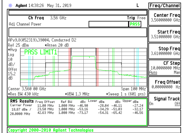
LTE B48 20MHz QPSK Low Channel RB100-0
