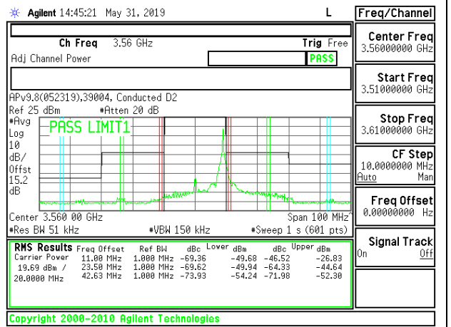
LTE B48 20MHz 16QAM Low Channel RB1-99
