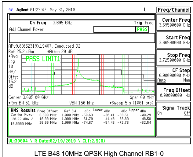
LTE B48 10MHz QPSK High Channel RB1-0
