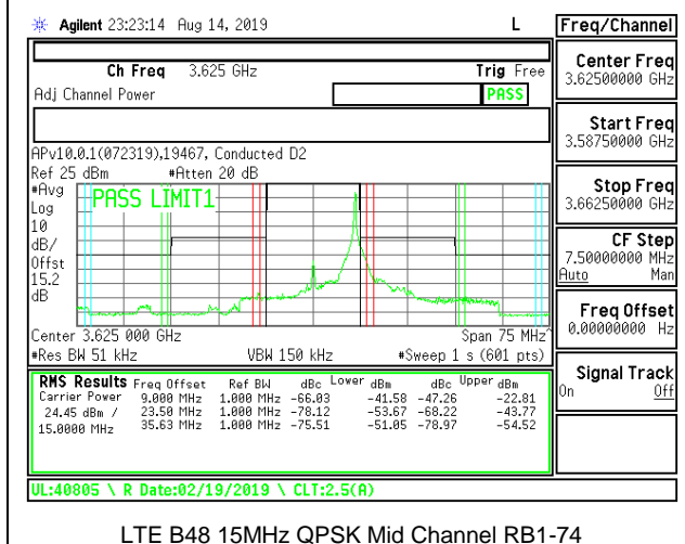
LTE B48 15MHz QPSK Mid Channel RB1-74
