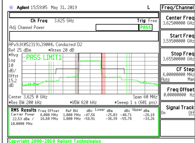
LTE B48 10MHz QPSK Mid Channel RB50-0
