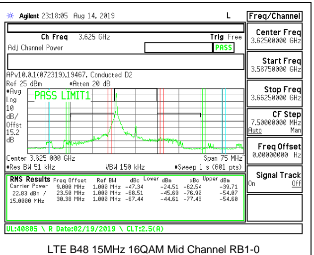
LTE B48 15MHz 16QAM Mid Channel RB1-0
