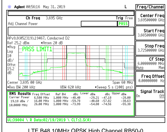
LTE B48 10MHz QPSK High Channel RB50-0
