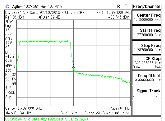
LTE B66 3MHz QPSK High Channel RB15-0
