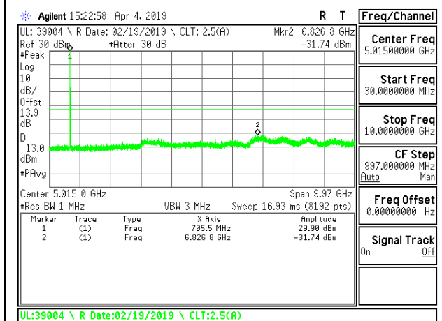
LTE B17 10MHz QPSK Middle Channel RB1-0
