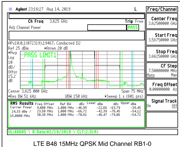
LTE B48 15MHz QPSK Mid Channel RB1-0
