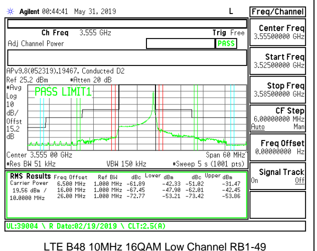
LTE B48 10MHz 16QAM Low Channel RB1-49
