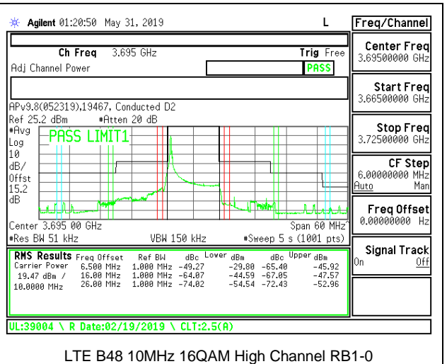
LTE B48 10MHz 16QAM High Channel RB1-0
