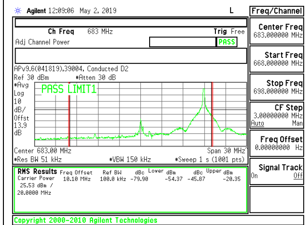
LTE B71 20MHz QPSK Middle Channel RB1-99
