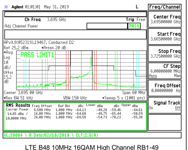
LTE B48 10MHz 16QAM High Channel RB1-49
