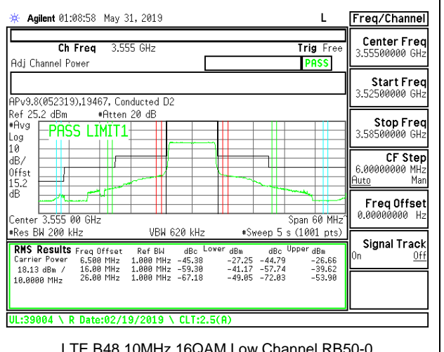
LTE B48 10MHz 16QAM Low Channel RB50-0
