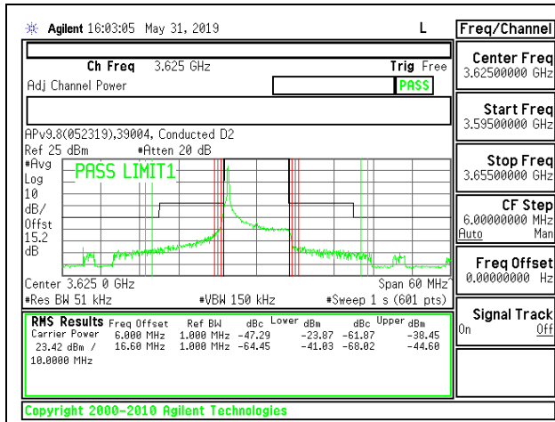
LTE B48 10MHz QPSK Mid Channel RB1-0
