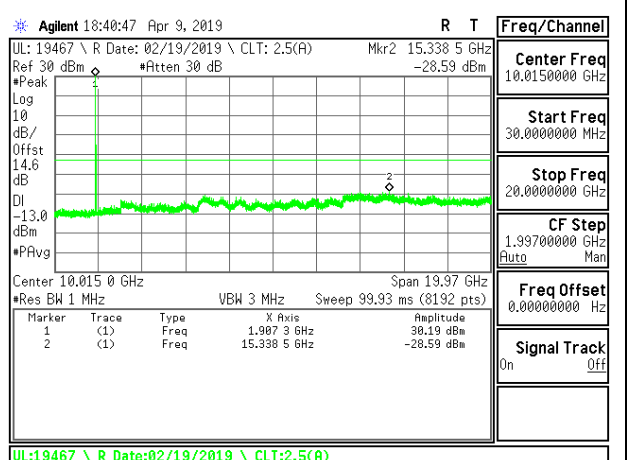
LTE B2 3MHz 16QAM High Channel RB1-0
