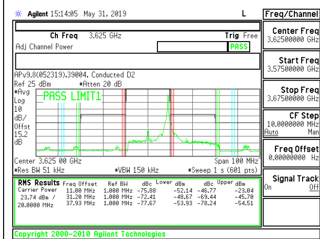
LTE B48 20MHz QPSK Mid Channel RB1-99
