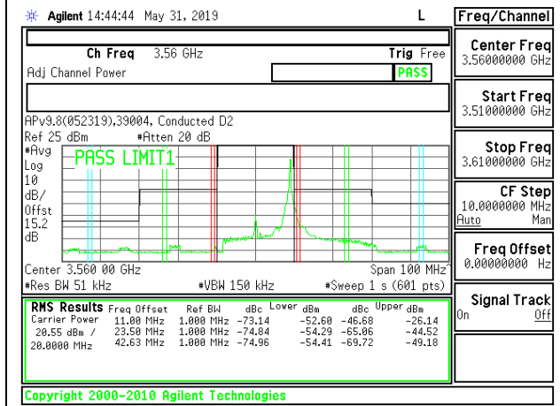
LTE B48 20MHz QPSK Low Channel RB1-99
