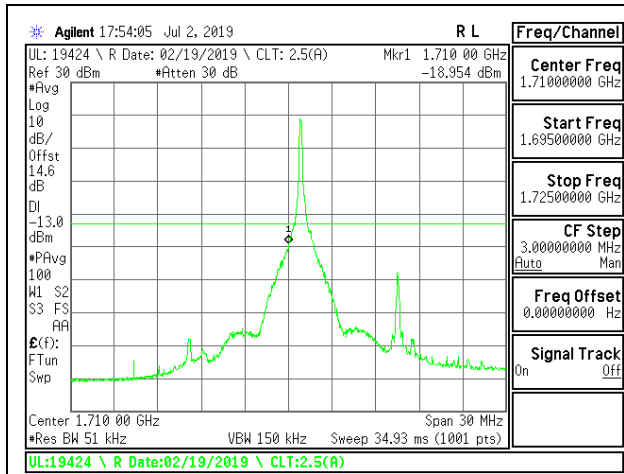
LTE B66 15MHz 16QAM Low Channel RB1-0 not the peak one
