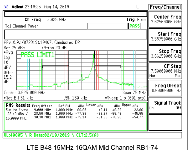
LTE B48 15MHz 16QAM Mid Channel RB1-74
