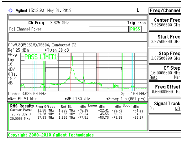
LTE B48 20MHz QPSK Mid Channel RB1-0
