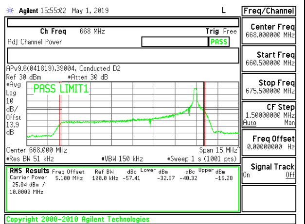
LTE B71 10MHz 16QAM Low Channel RB1-49
