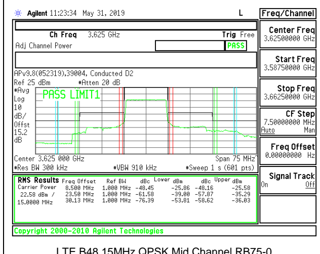
LTE B48 15MHz QPSK Mid Channel RB75-0
