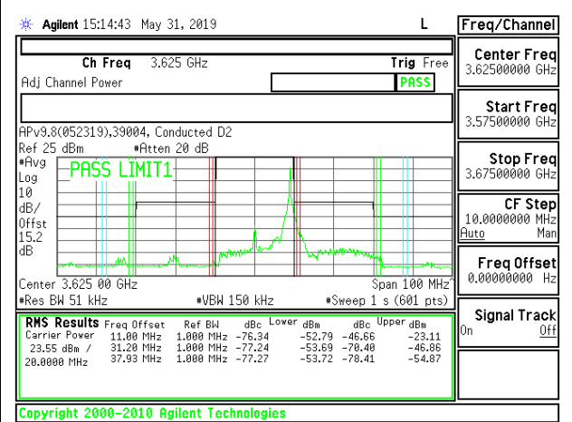
LTE B48 20MHz 16QAM Mid Channel RB1-99
