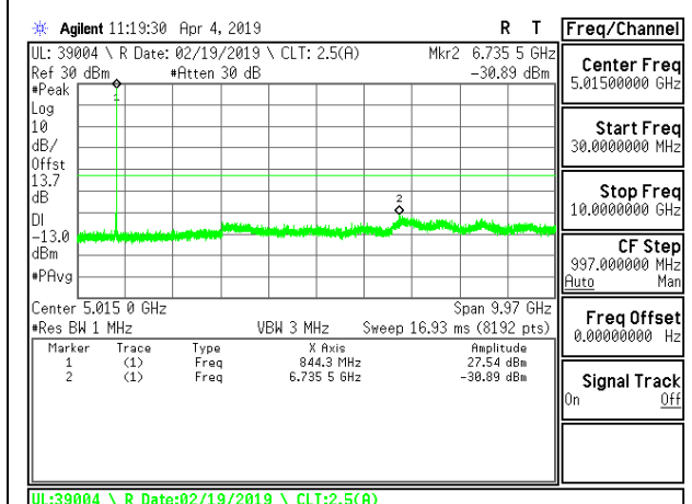
LTE B5 5MHz QPSK High Channel RB1-0
