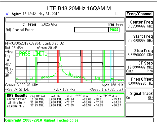
LTE B48 20MHz 16QAM Mid Channel RB1-0
