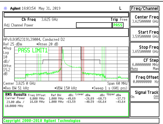
LTE B48 10MHz 16QAM Mid Channel RB1-0
