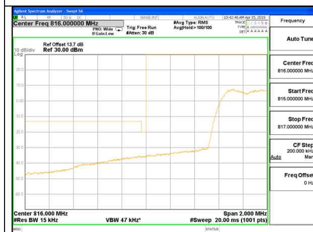
CDMA BC10 1xEV-DO Rev A Low Channel, RBW=1% of EBW ID:39919
