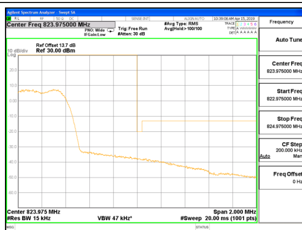
CDMA BC10 1xRTT High Channel, RBW=1% of EBW ID:39919
