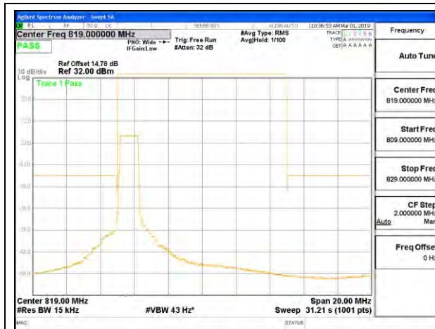
LTE B26 1.4MHz 16QAM Low Channel RB6-0 ID:12491
