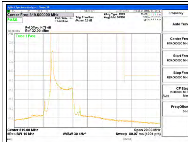
LTE B26 3MHz 16QAM Low Channel RB1-0 ID:12491
