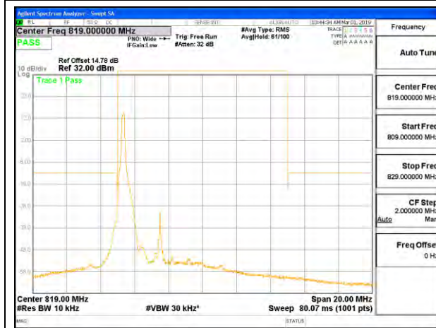
LTE B26 5MHz QPSK Low Channel RB1-0 ID:12491
