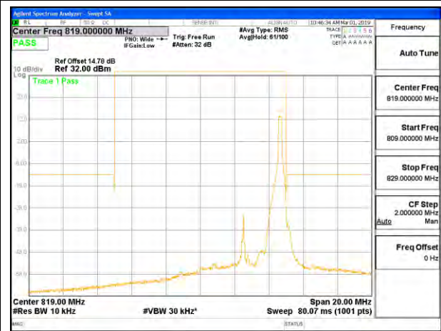
LTE B26 5MHz QPSK High Channel RB1-24 ID:12491
