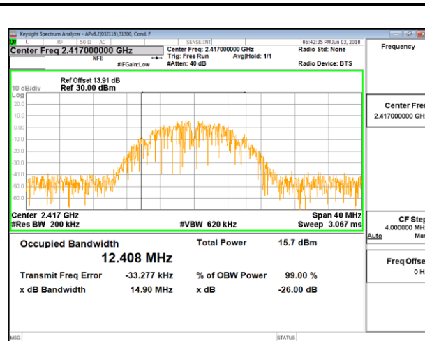
LOW CHANNEL 2
