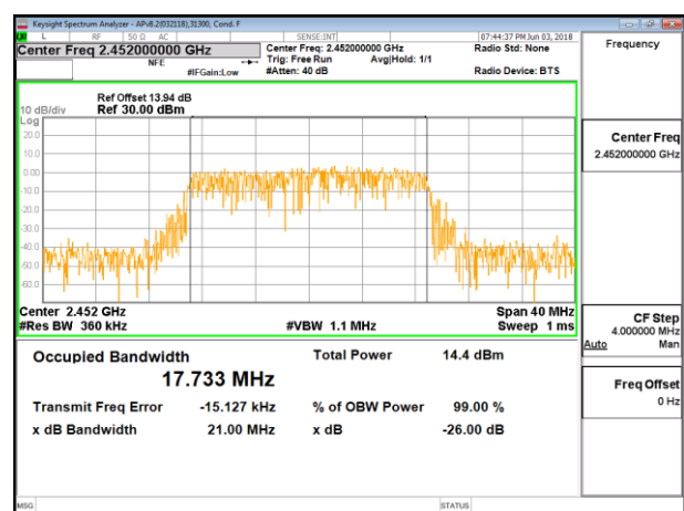
HIGH CHANNEL 9
