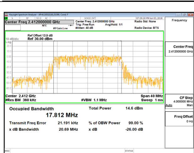
LOW CHANNEL 1
