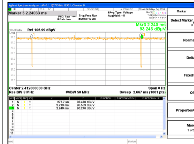
DUTY CYCLE 802.11n HT20 CDD MODE
