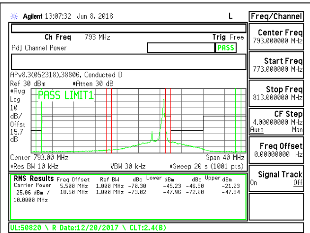
LTE B14 5MHz 16QAM High Channel RB1-24
