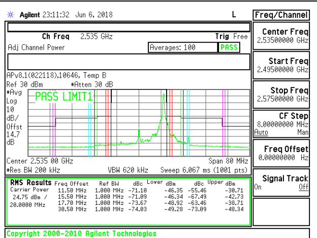
LTE B7 20MHz 16QAM Middle Channel RB1-99
