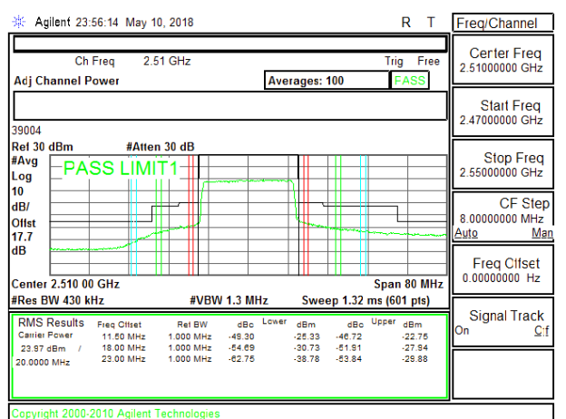
LTE B7 20MHz 16QAM Low Channel RB100-0
