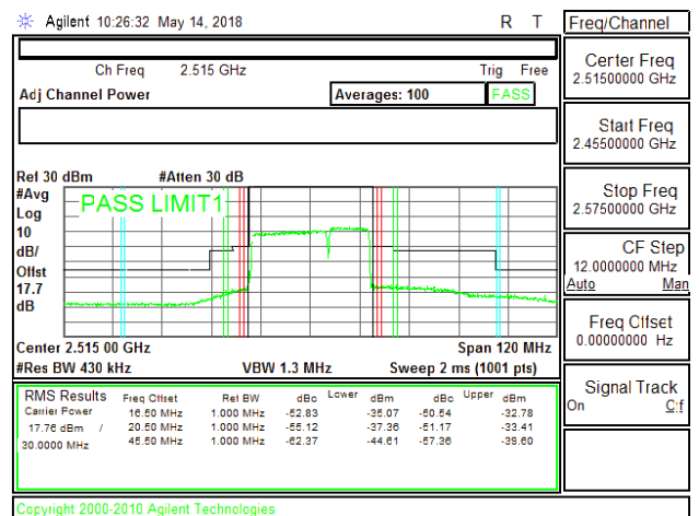
LTE B7 20MHz + 10MHz 16QAM Low Ch RB100-0 + RB50-0 ID10643
