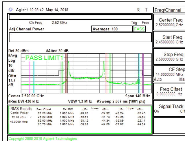
LTE B7 20MHz + 20MHz 16QAM Low Ch RB1-0 + RB1-99 ID10643
