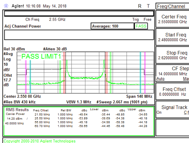
LTE B7 20MHz + 20MHz 16QAM High Ch RB1-0 + RB1-99 ID10643
