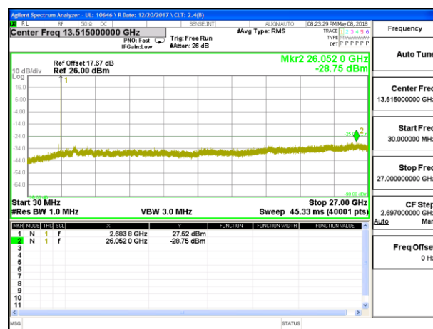
LTE B41 20MHz + 5MHz QPSK High Ch RB1-99 + RB1-0
