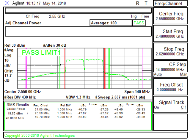
LTE B7 20MHz + 20MHz 16QAM High Ch RB100-0 + RB100-0 ID10643
