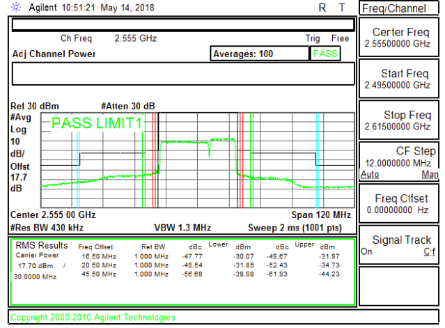
LTE B7 20MHz + 10MHz 16QAM High Ch RB100-0 + RB50-0 ID10643
