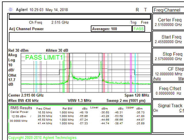
LTE B7 20MHz + 10MHz 16QAM Low Ch RB1-0 + RB1-49 ID10643
