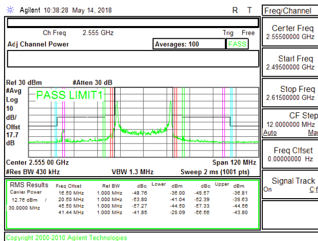
LTE B7 20MHz + 10MHz 16QAM High Ch RB1-0 + RB1-49 ID10643
