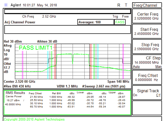
LTE B7 20MHz + 20MHz 16QAM Low Ch RB100-0 + RB100-0 ID10643
