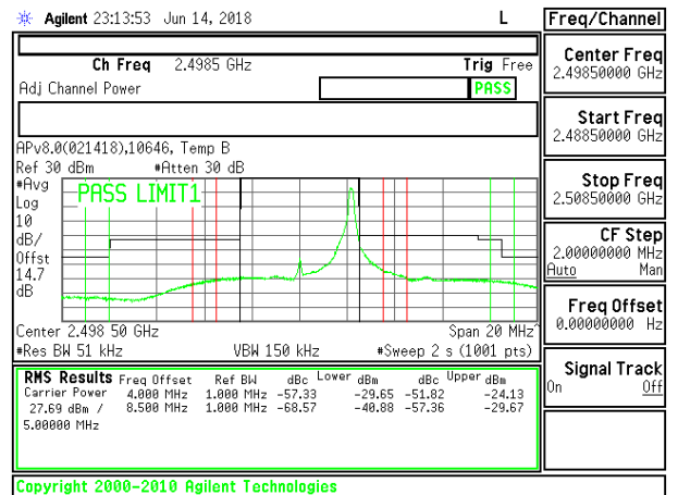
LTE B41 5MHz 16QAM Low Channel RB1-24
