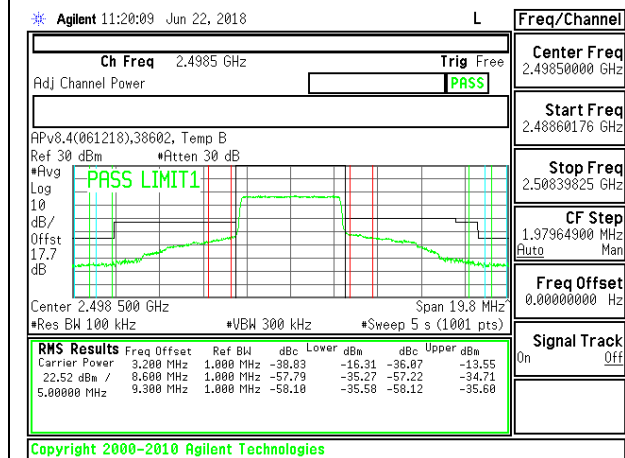
LTE B41 5MHz QPSK Low Channel RB25-0
