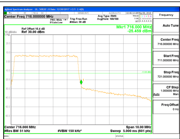
LTE B17 5MHz 16QAM High Channel RB25-0
