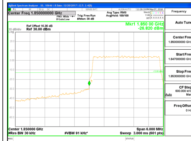
LTE B25 3MHz 16QAM Low Channel RB15-0
