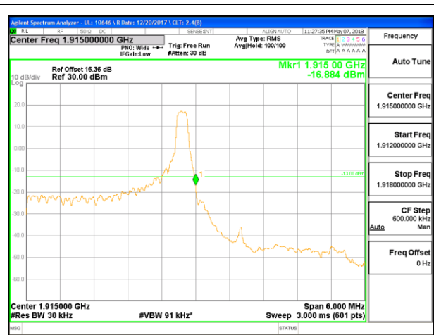
LTE B25 3MHz 16QAM High Channel RB1-14
