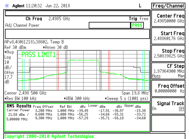
LTE B41 5MHz 16QAM Low Channel RB25-0
