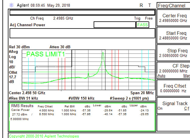
LTE B41 5MHz QPSK Low Channel RB1-24
